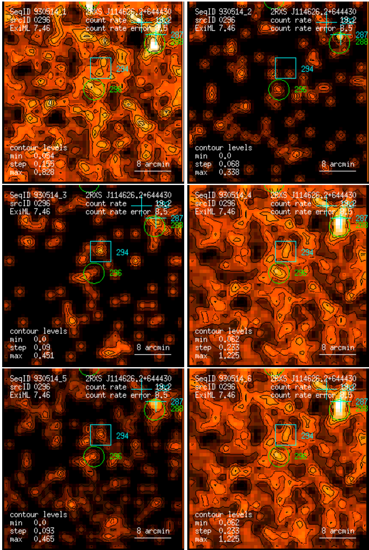
Figure 296: RASS 930514: detection 0296: band rate images, Gaussian filter: (1) PSPC channels 11 – 41, (2) 52 – 90, (3) 91 – 201, (4) 11 – 235, (5) 52 – 201, (6) 11 – 201. Broad band rates in counts/ks. Band rate contour levels in counts/ks/arcmin 2 .
