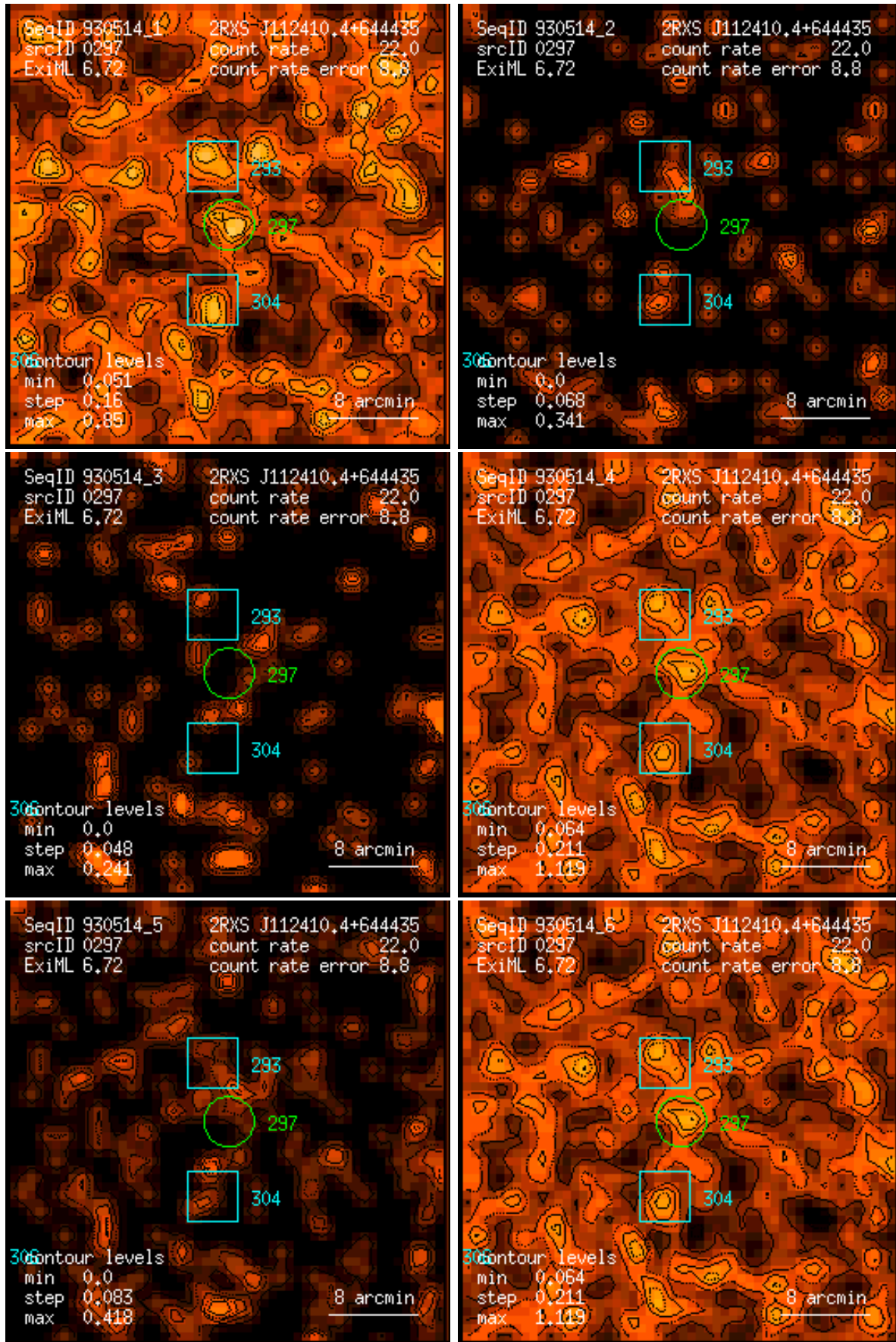
Figure 297: RASS 930514: detection 0297: band rate images, Gaussian filter: (1) PSPC channels 11 – 41, (2) 52 – 90, (3) 91 – 201, (4) 11 – 235, (5) 52 – 201, (6) 11 – 201. Broad band rates in counts/ks. Band rate contour levels in counts/ks/arcmin 2 .
