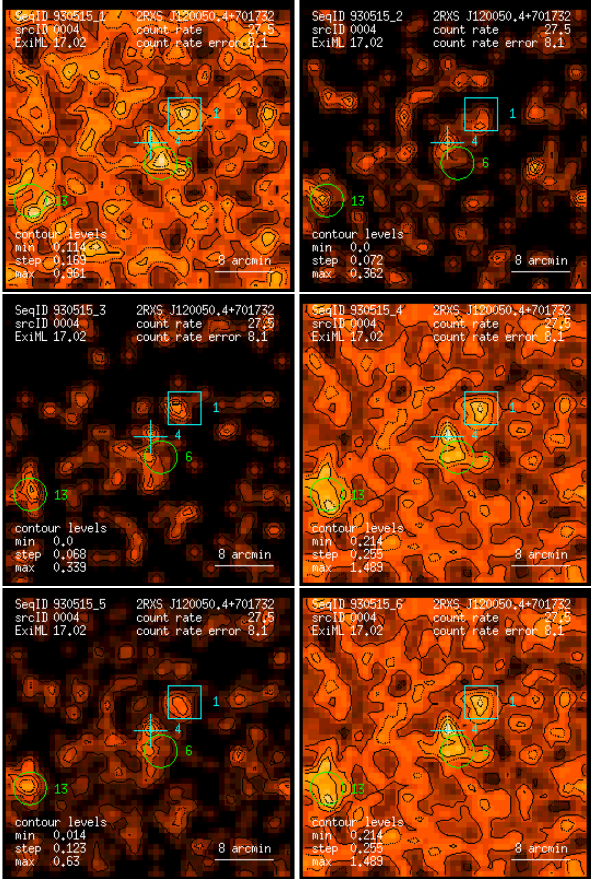
Figure 4: RASS 930515: detection 0004: band rate images, Gaussian filter: (1) PSPC channels 11 – 41, (2) 52 – 90, (3) 91 – 201, (4) 11 – 235, (5) 52 – 201, (6) 11 – 201. Broad band rates in counts/ks. Band rate contour levels in counts/ks/arcmin 2 .
