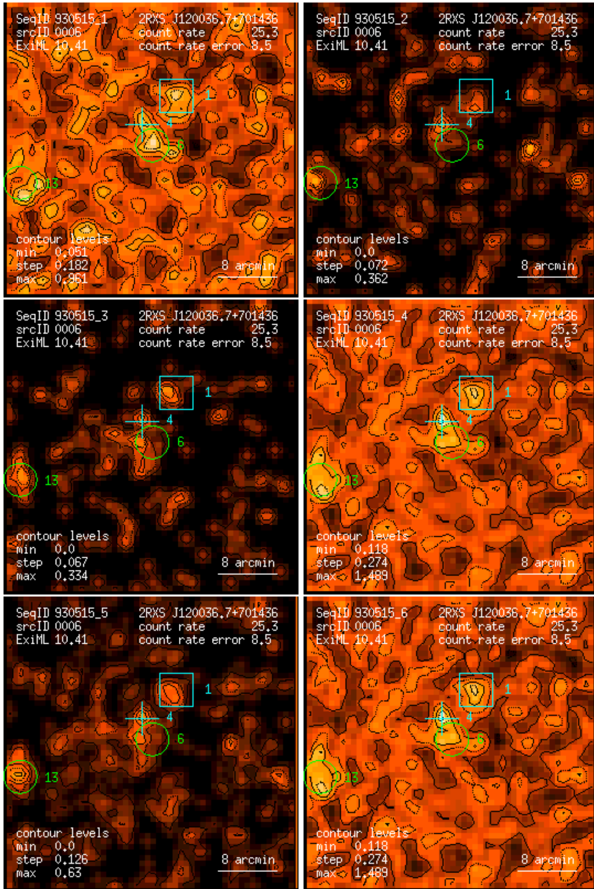
Figure 6: RASS 930515: detection 0006: band rate images, Gaussian filter: (1) PSPC channels 11 – 41, (2) 52 – 90, (3) 91 – 201, (4) 11 – 235, (5) 52 – 201, (6) 11 – 201. Broad band rates in counts/ks. Band rate contour levels in counts/ks/arcmin 2 .
