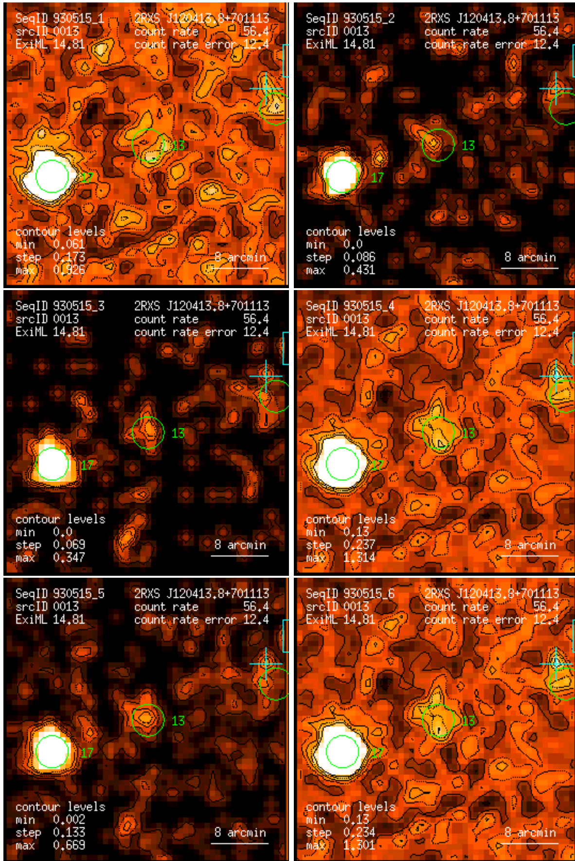
Figure 13: RASS 930515: detection 0013: band rate images, Gaussian filter: (1) PSPC channels 11 – 41, (2) 52 – 90, (3) 91 – 201, (4) 11 – 235, (5) 52 – 201, (6) 11 – 201. Broad band rates in counts/ks. Band rate contour levels in counts/ks/arcmin 2 .
