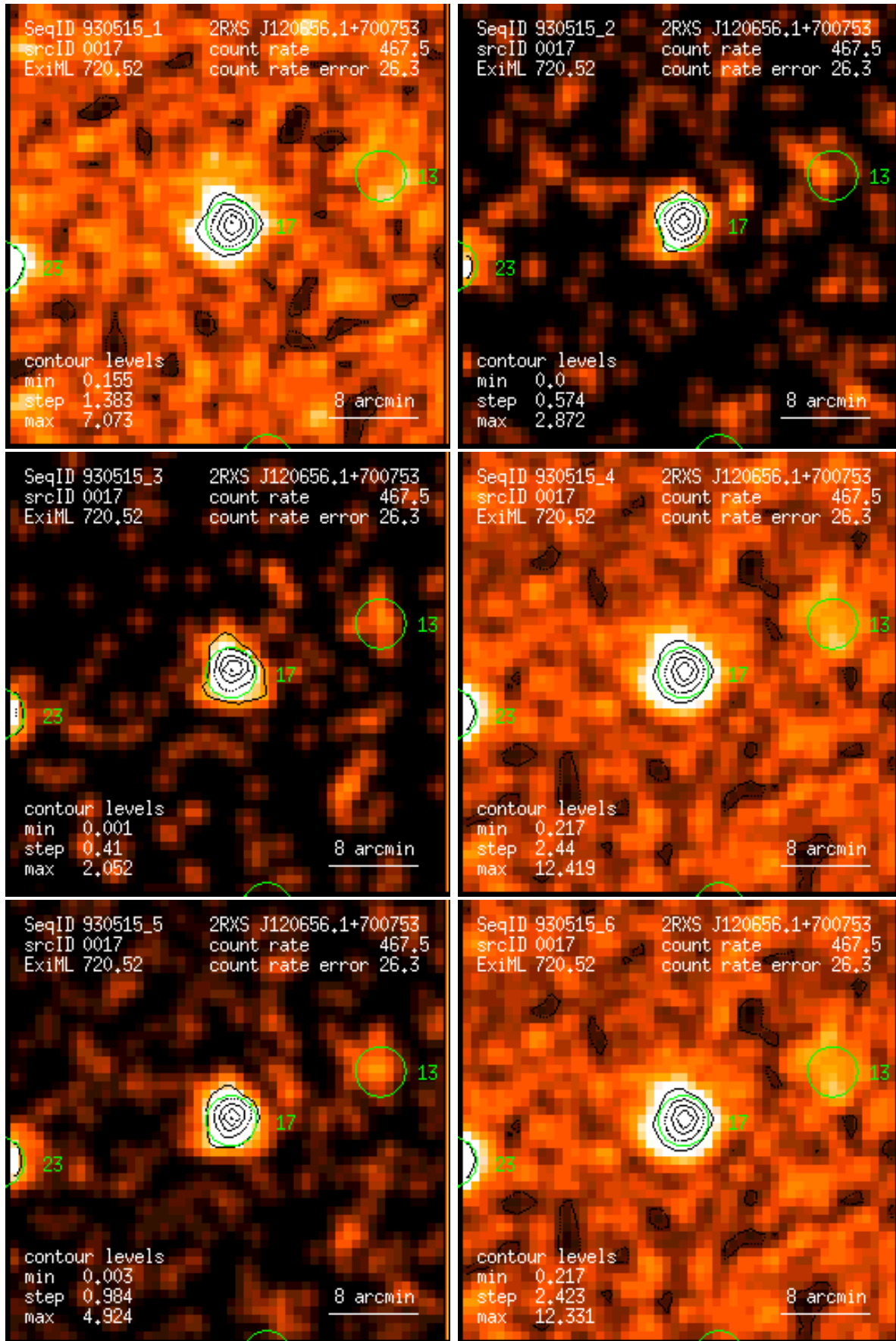
Figure 17: RASS 930515: detection 0017: band rate images, Gaussian filter: (1) PSPC channels 11 – 41, (2) 52 – 90, (3) 91 – 201, (4) 11 – 235, (5) 52 – 201, (6) 11 – 201. Broad band rates in counts/ks. Band rate contour levels in counts/ks/arcmin 2 .
