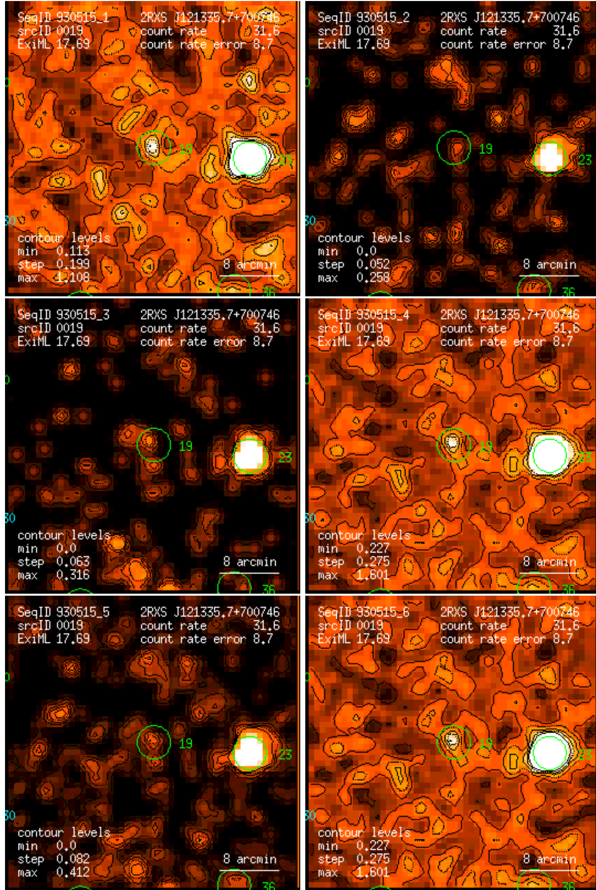
Figure 19: RASS 930515: detection 0019: band rate images, Gaussian filter: (1) PSPC channels 11 – 41, (2) 52 – 90, (3) 91 – 201, (4) 11 – 235, (5) 52 – 201, (6) 11 – 201. Broad band rates in counts/ks. Band rate contour levels in counts/ks/arcmin 2 .
