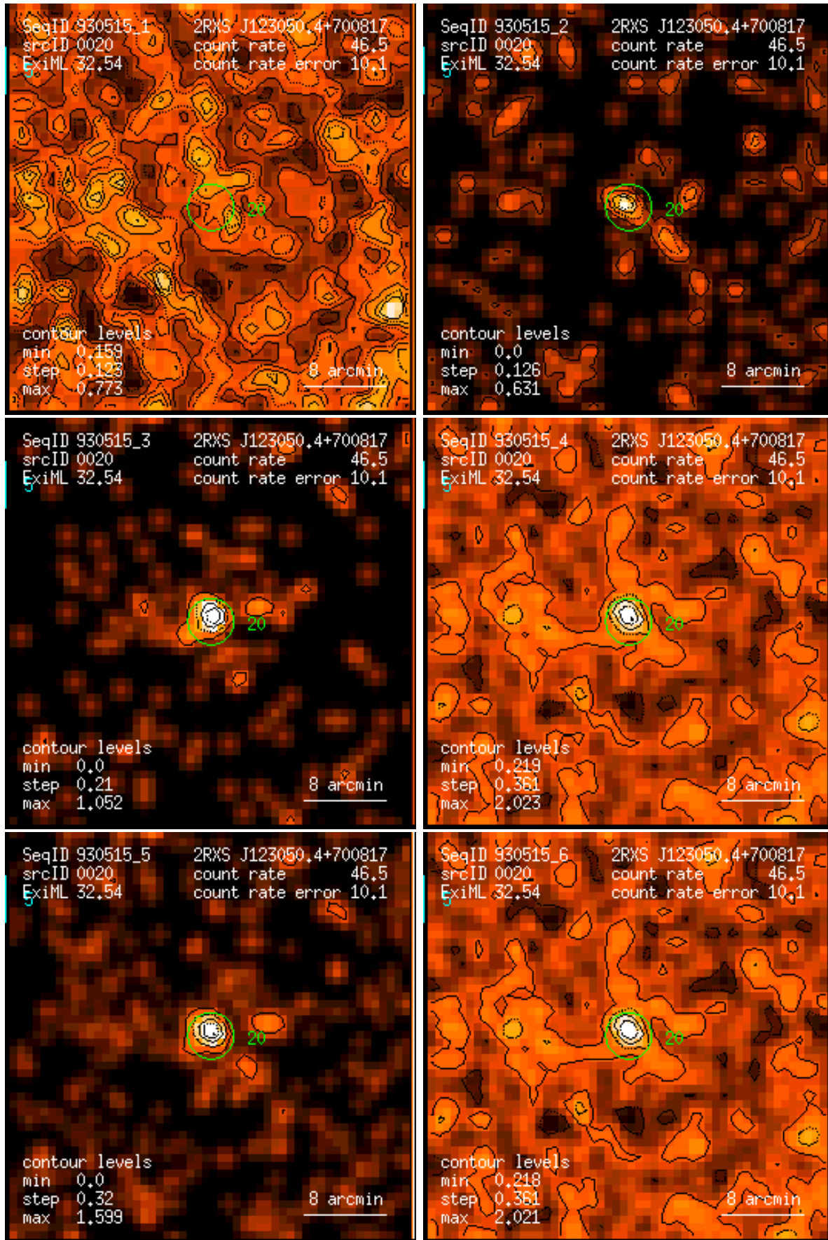
Figure 20: RASS 930515: detection 0020: band rate images, Gaussian filter: (1) PSPC channels 11 – 41, (2) 52 – 90, (3) 91 – 201, (4) 11 – 235, (5) 52 – 201, (6) 11 – 201. Broad band rates in counts/ks. Band rate contour levels in counts/ks/arcmin 2 .
