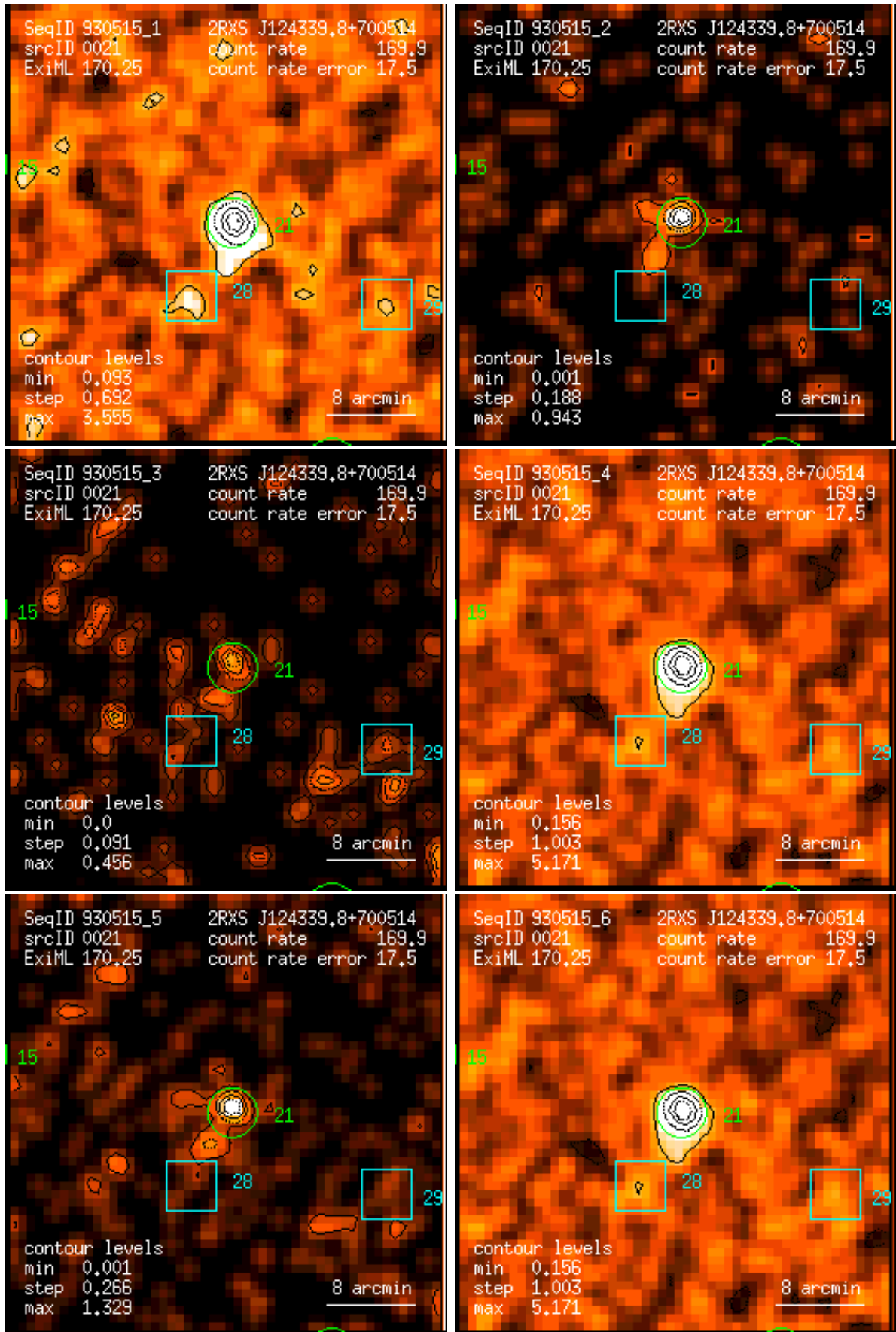
Figure 21: RASS 930515: detection 0021: band rate images, Gaussian filter: (1) PSPC channels 11 – 41, (2) 52 – 90, (3) 91 – 201, (4) 11 – 235, (5) 52 – 201, (6) 11 – 201. Broad band rates in counts/ks. Band rate contour levels in counts/ks/arcmin 2 .
