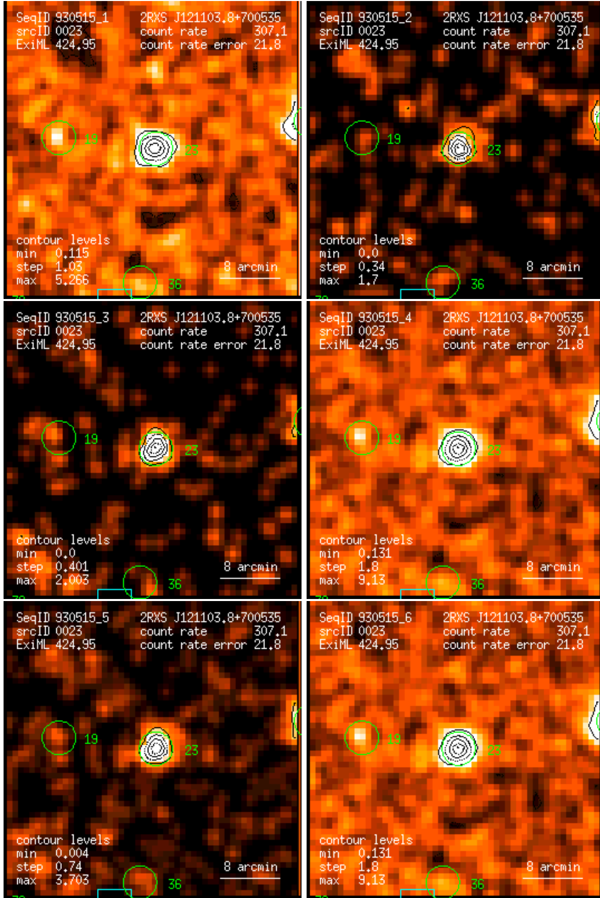
Figure 23: RASS 930515: detection 0023: band rate images, Gaussian filter: (1) PSPC channels 11 – 41, (2) 52 – 90, (3) 91 – 201, (4) 11 – 235, (5) 52 – 201, (6) 11 – 201. Broad band rates in counts/ks. Band rate contour levels in counts/ks/arcmin 2 .
