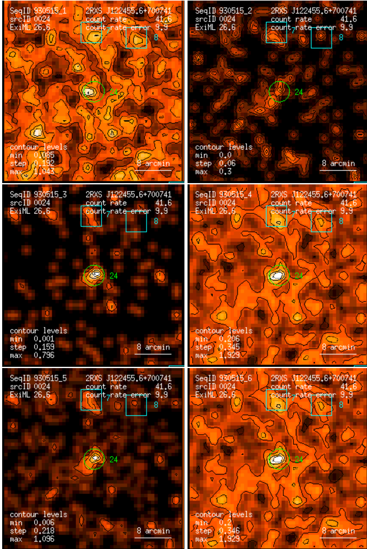
Figure 24: RASS 930515: detection 0024: band rate images, Gaussian filter: (1) PSPC channels 11 – 41, (2) 52 – 90, (3) 91 – 201, (4) 11 – 235, (5) 52 – 201, (6) 11 – 201. Broad band rates in counts/ks. Band rate contour levels in counts/ks/arcmin 2 .
