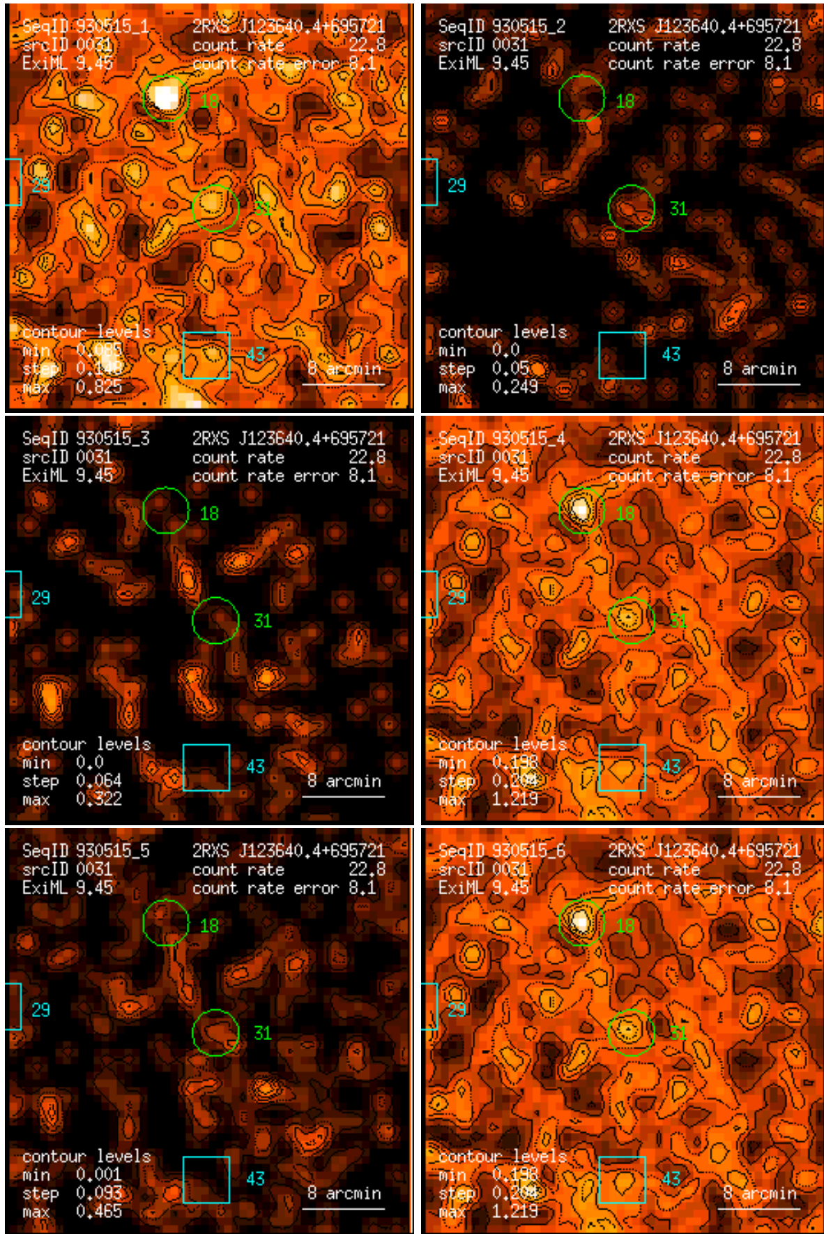
Figure 31: RASS 930515: detection 0031: band rate images, Gaussian filter: (1) PSPC channels 11 – 41, (2) 52 – 90, (3) 91 – 201, (4) 11 – 235, (5) 52 – 201, (6) 11 – 201. Broad band rates in counts/ks. Band rate contour levels in counts/ks/arcmin 2 .
