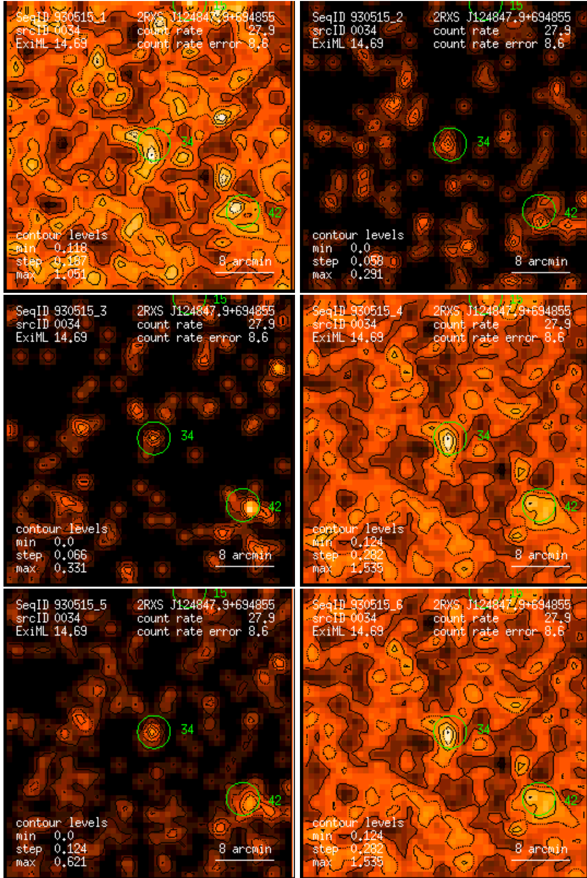
Figure 34: RASS 930515: detection 0034: band rate images, Gaussian filter: (1) PSPC channels 11 – 41, (2) 52 – 90, (3) 91 – 201, (4) 11 – 235, (5) 52 – 201, (6) 11 – 201. Broad band rates in counts/ks. Band rate contour levels in counts/ks/arcmin 2 .
