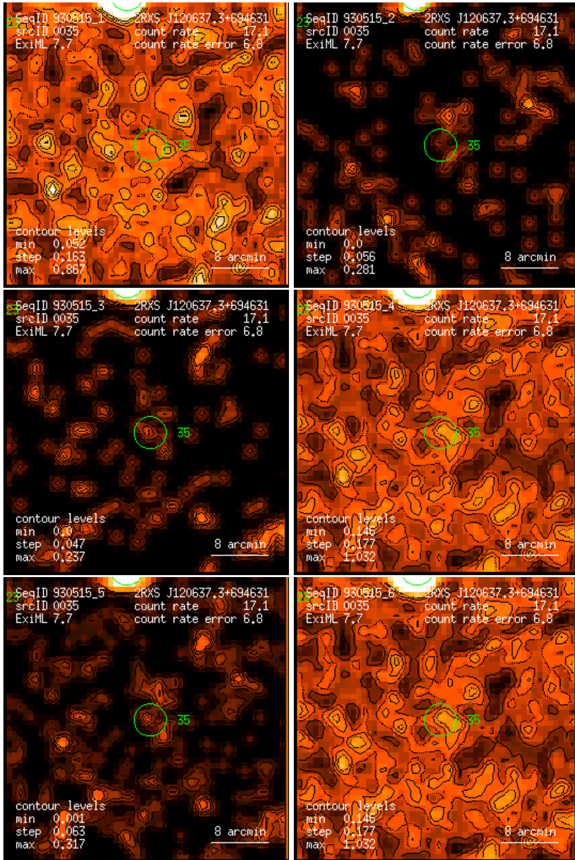
Figure 35: RASS 930515: detection 0035: band rate images, Gaussian filter: (1) PSPC channels 11 – 41, (2) 52 – 90, (3) 91 – 201, (4) 11 – 235, (5) 52 – 201, (6) 11 – 201. Broad band rates in counts/ks. Band rate contour levels in counts/ks/arcmin 2 .
