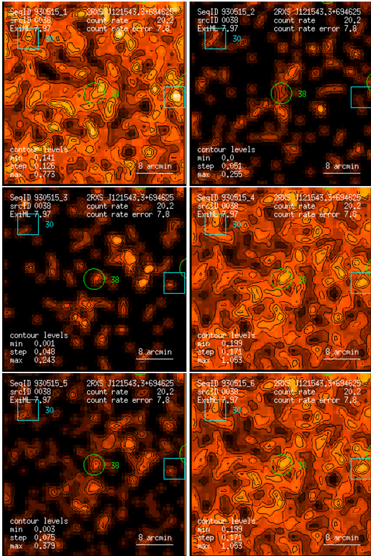
Figure 38: RASS 930515: detection 0038: band rate images, Gaussian filter: (1) PSPC channels 11 – 41, (2) 52 – 90, (3) 91 – 201, (4) 11 – 235, (5) 52 – 201, (6) 11 – 201. Broad band rates in counts/ks. Band rate contour levels in counts/ks/arcmin 2 .
