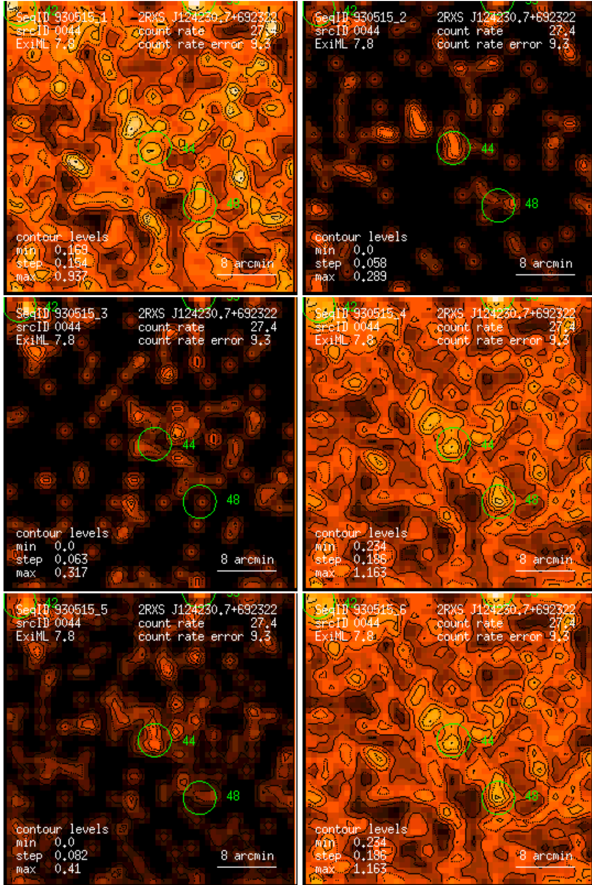
Figure 44: RASS 930515: detection 0044: band rate images, Gaussian filter: (1) PSPC channels 11 – 41, (2) 52 – 90, (3) 91 – 201, (4) 11 – 235, (5) 52 – 201, (6) 11 – 201. Broad band rates in counts/ks. Band rate contour levels in counts/ks/arcmin 2 .
