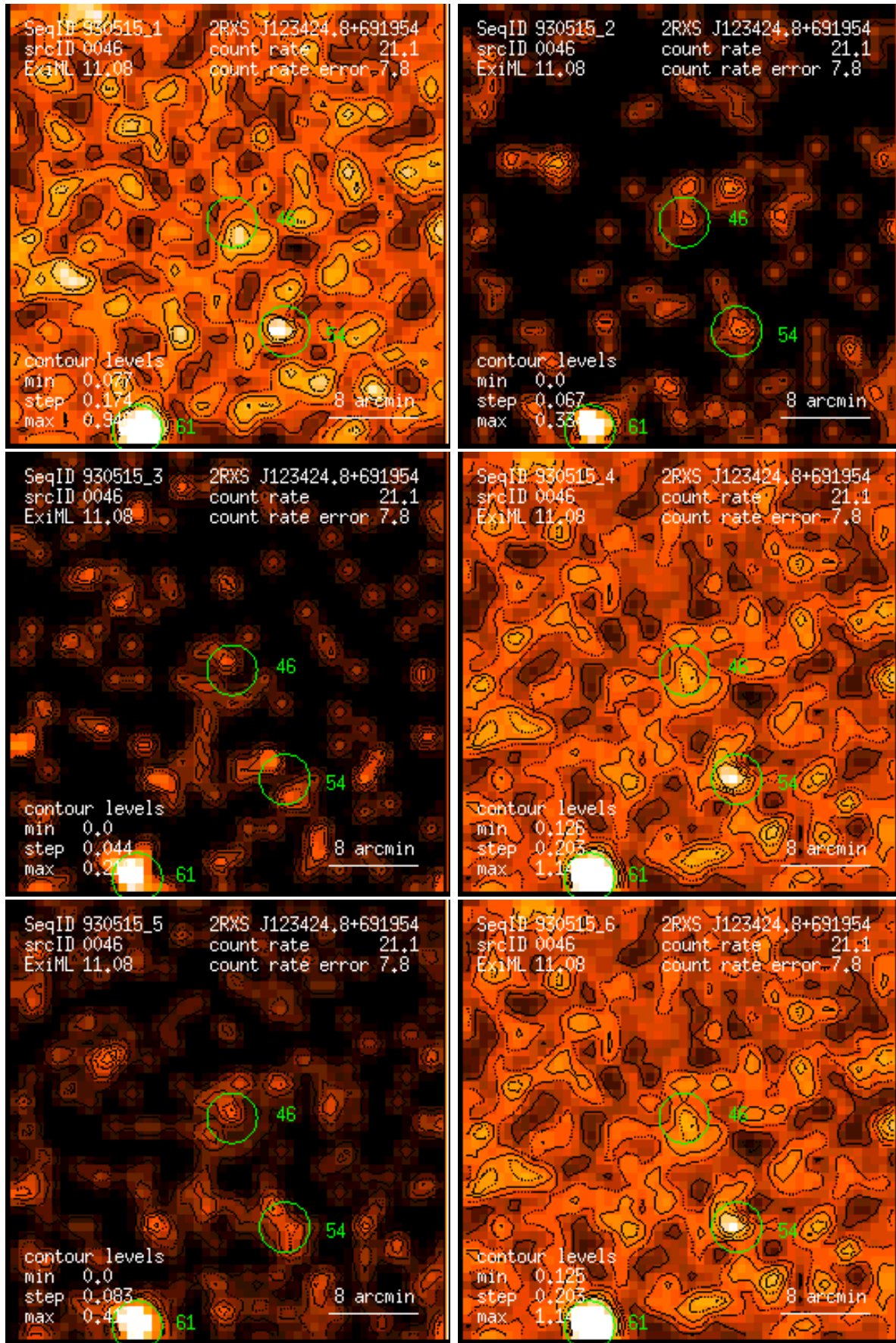
Figure 46: RASS 930515: detection 0046: band rate images, Gaussian filter: (1) PSPC channels 11 – 41, (2) 52 – 90, (3) 91 – 201, (4) 11 – 235, (5) 52 – 201, (6) 11 – 201. Broad band rates in counts/ks. Band rate contour levels in counts/ks/arcmin 2 .
