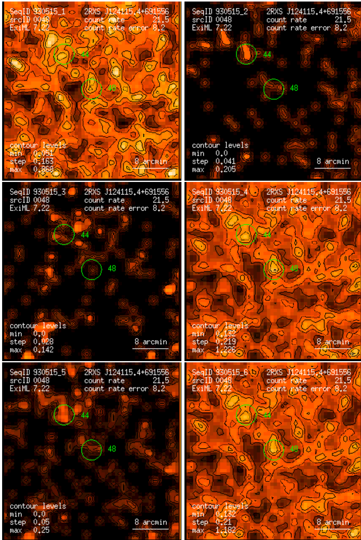
Figure 48: RASS 930515: detection 0048: band rate images, Gaussian filter: (1) PSPC channels 11 – 41, (2) 52 – 90, (3) 91 – 201, (4) 11 – 235, (5) 52 – 201, (6) 11 – 201. Broad band rates in counts/ks. Band rate contour levels in counts/ks/arcmin 2 .
