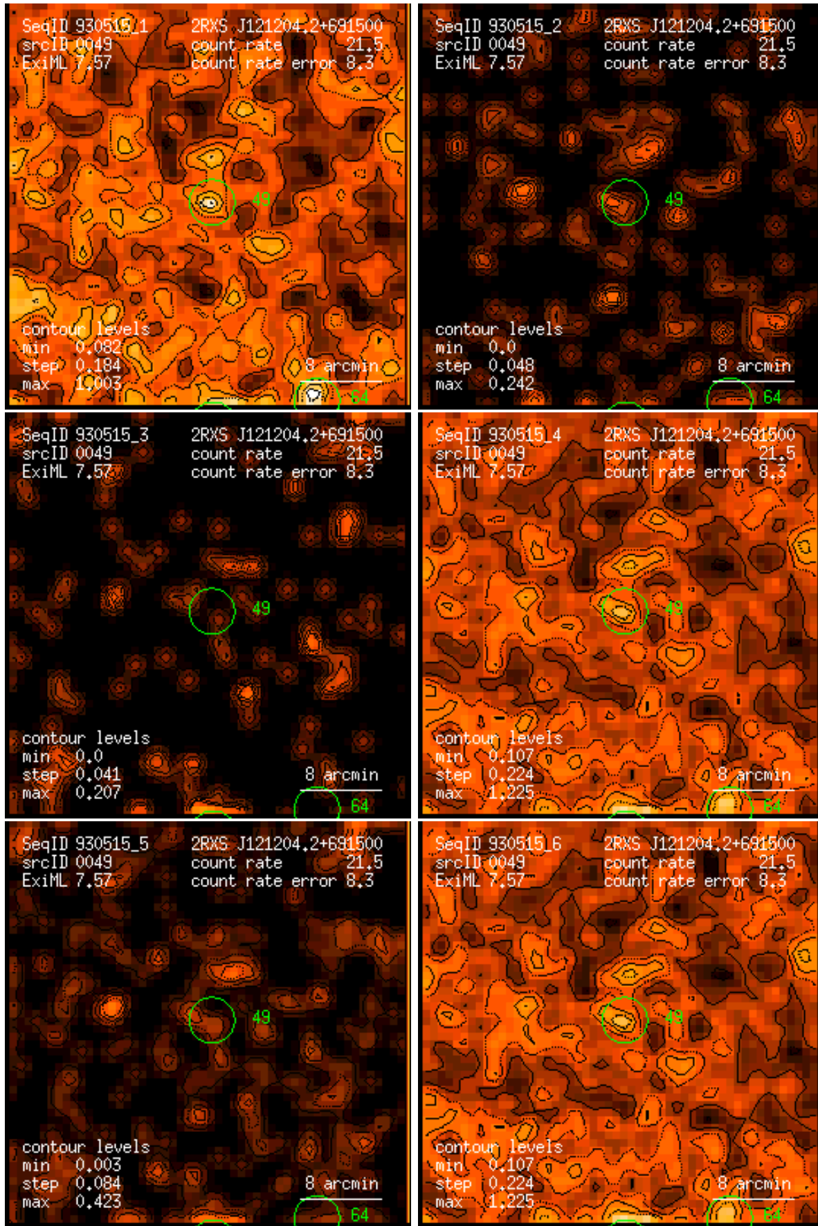
Figure 49: RASS 930515: detection 0049: band rate images, Gaussian filter: (1) PSPC channels 11 – 41, (2) 52 – 90, (3) 91 – 201, (4) 11 – 235, (5) 52 – 201, (6) 11 – 201. Broad band rates in counts/ks. Band rate contour levels in counts/ks/arcmin 2 .
