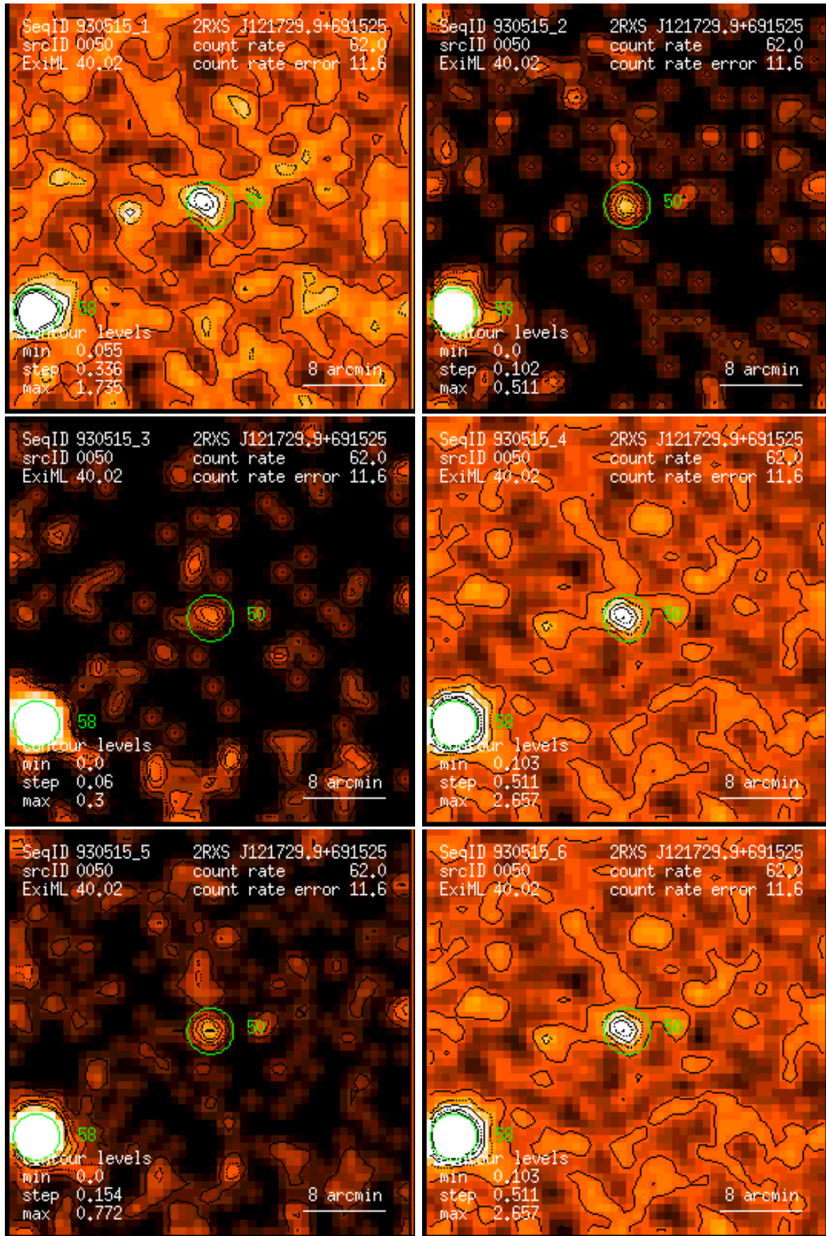
Figure 50: RASS 930515: detection 0050: band rate images, Gaussian filter: (1) PSPC channels 11 – 41, (2) 52 – 90, (3) 91 – 201, (4) 11 – 235, (5) 52 – 201, (6) 11 – 201. Broad band rates in counts/ks. Band rate contour levels in counts/ks/arcmin 2 .
