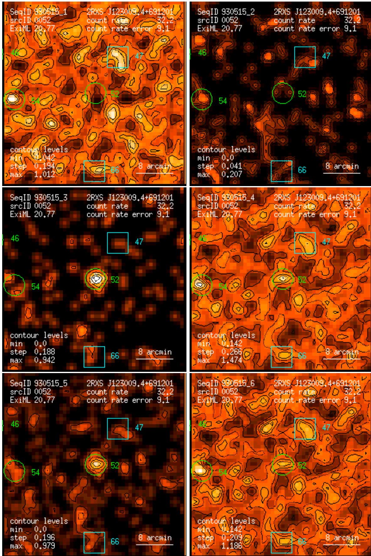
Figure 52: RASS 930515: detection 0052: band rate images, Gaussian filter: (1) PSPC channels 11 – 41, (2) 52 – 90, (3) 91 – 201, (4) 11 – 235, (5) 52 – 201, (6) 11 – 201. Broad band rates in counts/ks. Band rate contour levels in counts/ks/arcmin 2 .
