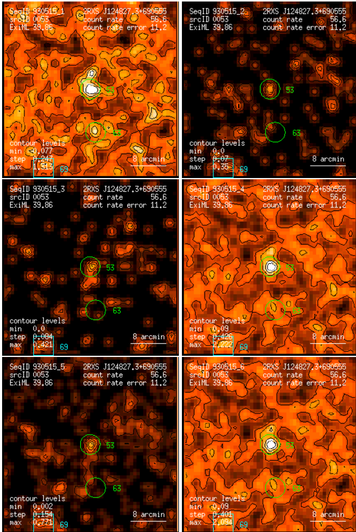
Figure 53: RASS 930515: detection 0053: band rate images, Gaussian filter: (1) PSPC channels 11 – 41, (2) 52 – 90, (3) 91 – 201, (4) 11 – 235, (5) 52 – 201, (6) 11 – 201. Broad band rates in counts/ks. Band rate contour levels in counts/ks/arcmin 2 .
