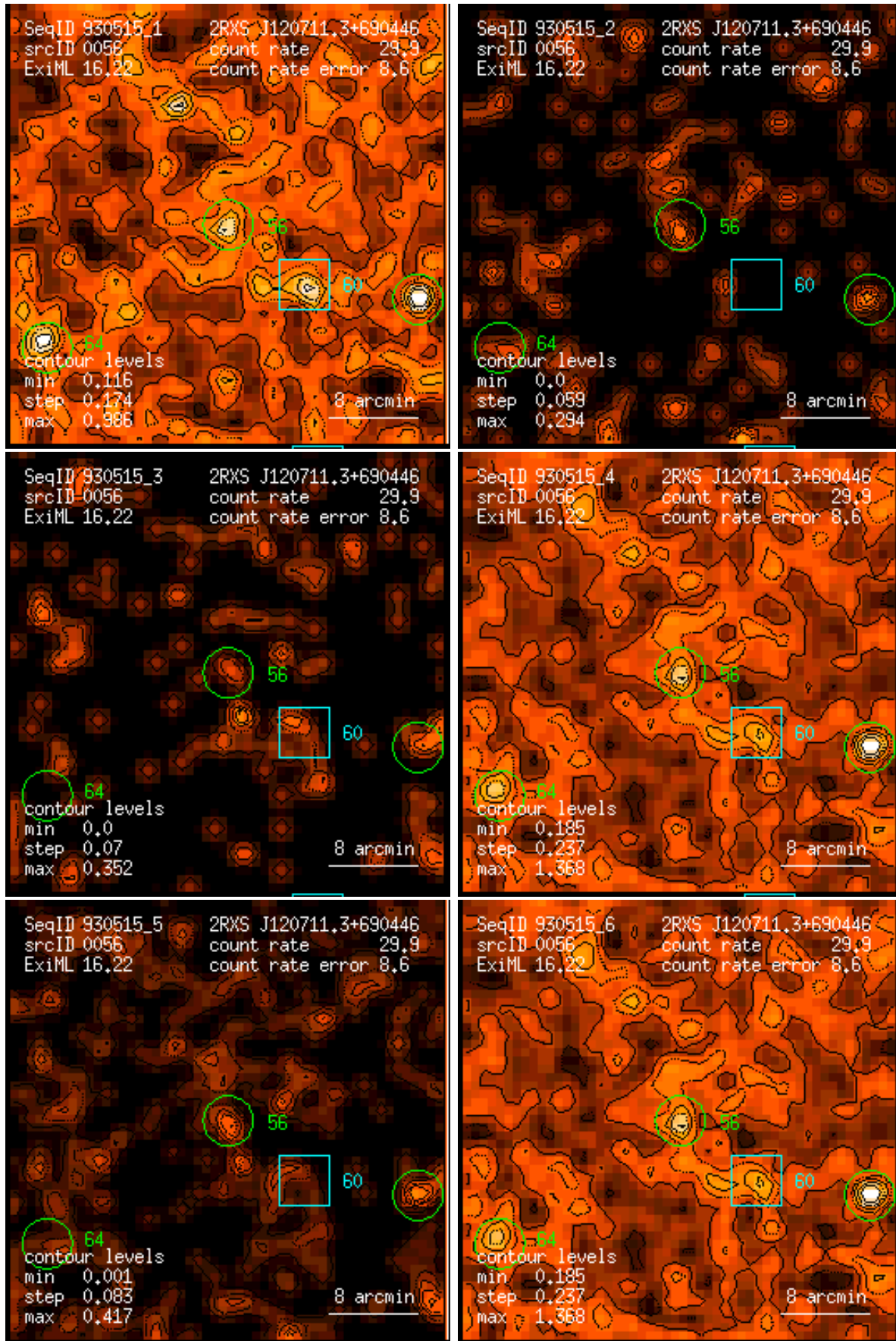
Figure 56: RASS 930515: detection 0056: band rate images, Gaussian filter: (1) PSPC channels 11 – 41, (2) 52 – 90, (3) 91 – 201, (4) 11 – 235, (5) 52 – 201, (6) 11 – 201. Broad band rates in counts/ks. Band rate contour levels in counts/ks/arcmin 2 .
