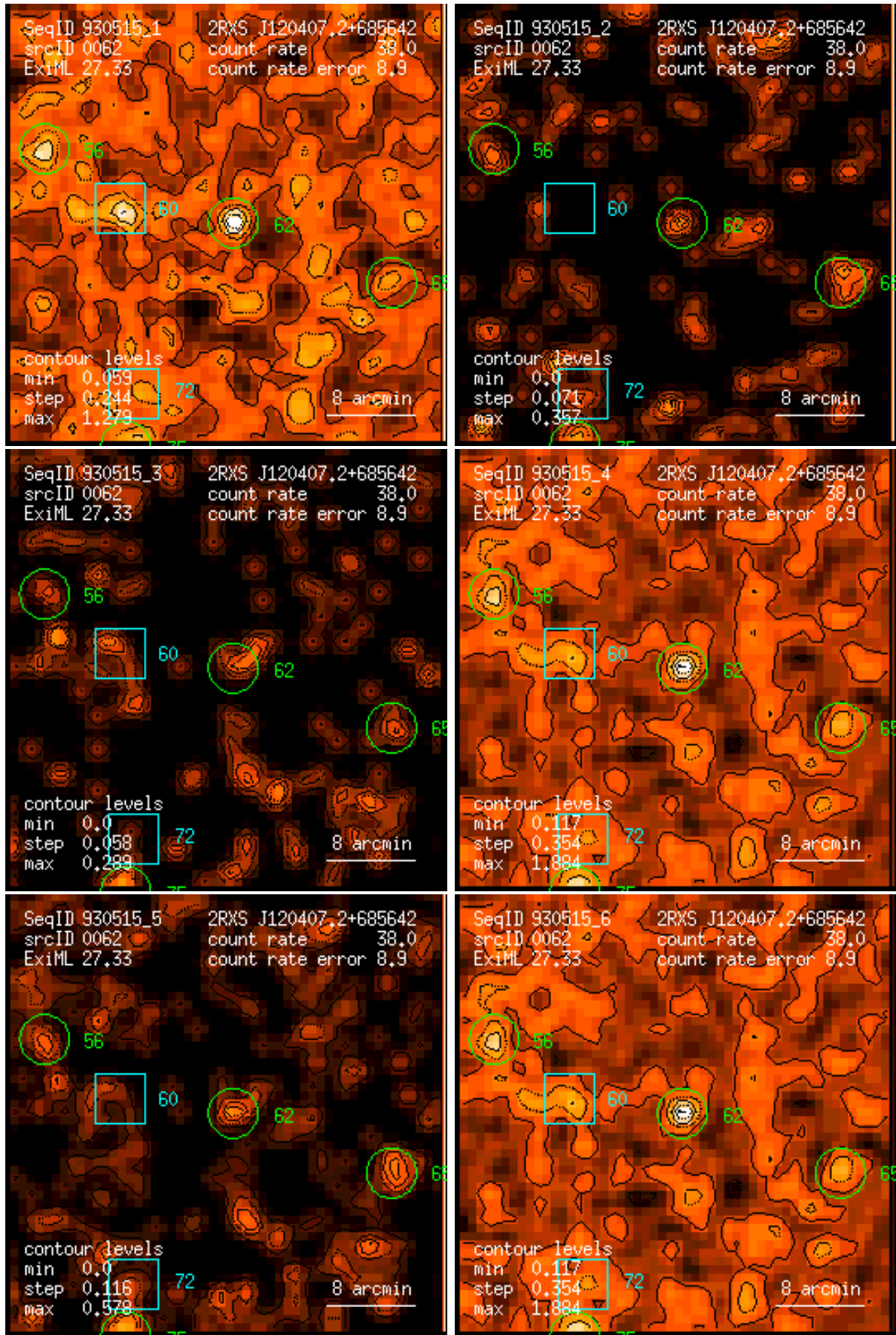
Figure 62: RASS 930515: detection 0062: band rate images, Gaussian filter: (1) PSPC channels 11 – 41, (2) 52 – 90, (3) 91 – 201, (4) 11 – 235, (5) 52 – 201, (6) 11 – 201. Broad band rates in counts/ks. Band rate contour levels in counts/ks/arcmin 2 .
