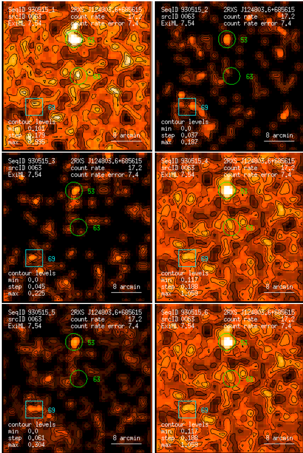
Figure 63: RASS 930515: detection 0063: band rate images, Gaussian filter: (1) PSPC channels 11 – 41, (2) 52 – 90, (3) 91 – 201, (4) 11 – 235, (5) 52 – 201, (6) 11 – 201. Broad band rates in counts/ks. Band rate contour levels in counts/ks/arcmin 2 .
