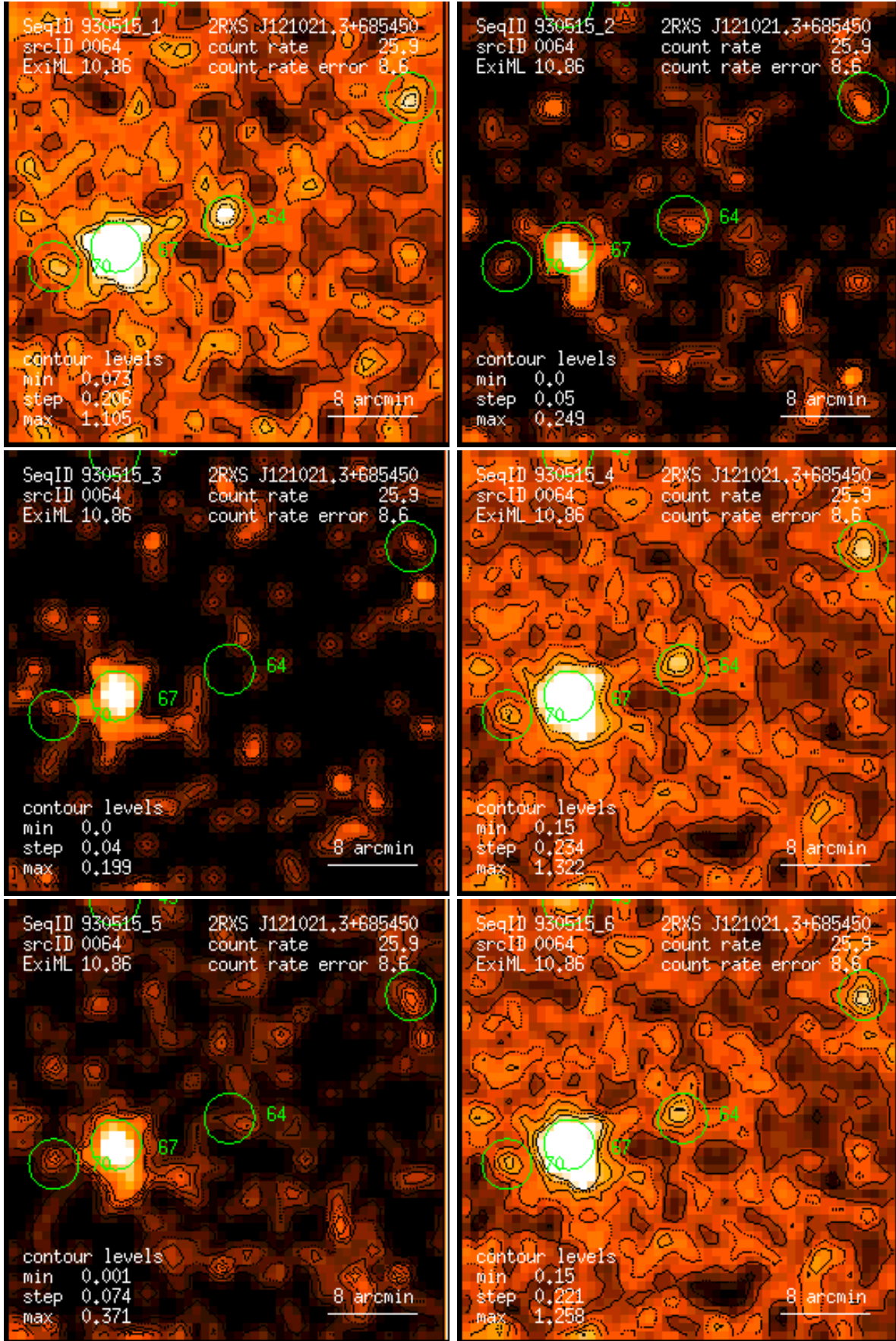
Figure 64: RASS 930515: detection 0064: band rate images, Gaussian filter: (1) PSPC channels 11 – 41, (2) 52 – 90, (3) 91 – 201, (4) 11 – 235, (5) 52 – 201, (6) 11 – 201. Broad band rates in counts/ks. Band rate contour levels in counts/ks/arcmin 2 .
