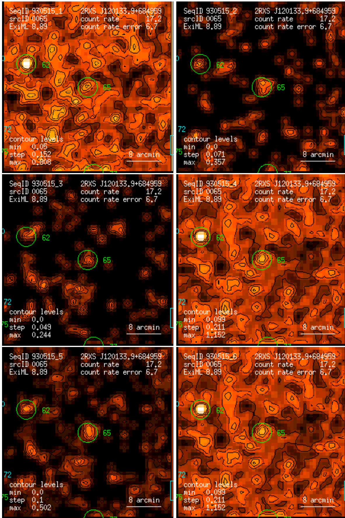
Figure 65: RASS 930515: detection 0065: band rate images, Gaussian filter: (1) PSPC channels 11 – 41, (2) 52 – 90, (3) 91 – 201, (4) 11 – 235, (5) 52 – 201, (6) 11 – 201. Broad band rates in counts/ks. Band rate contour levels in counts/ks/arcmin 2 .
