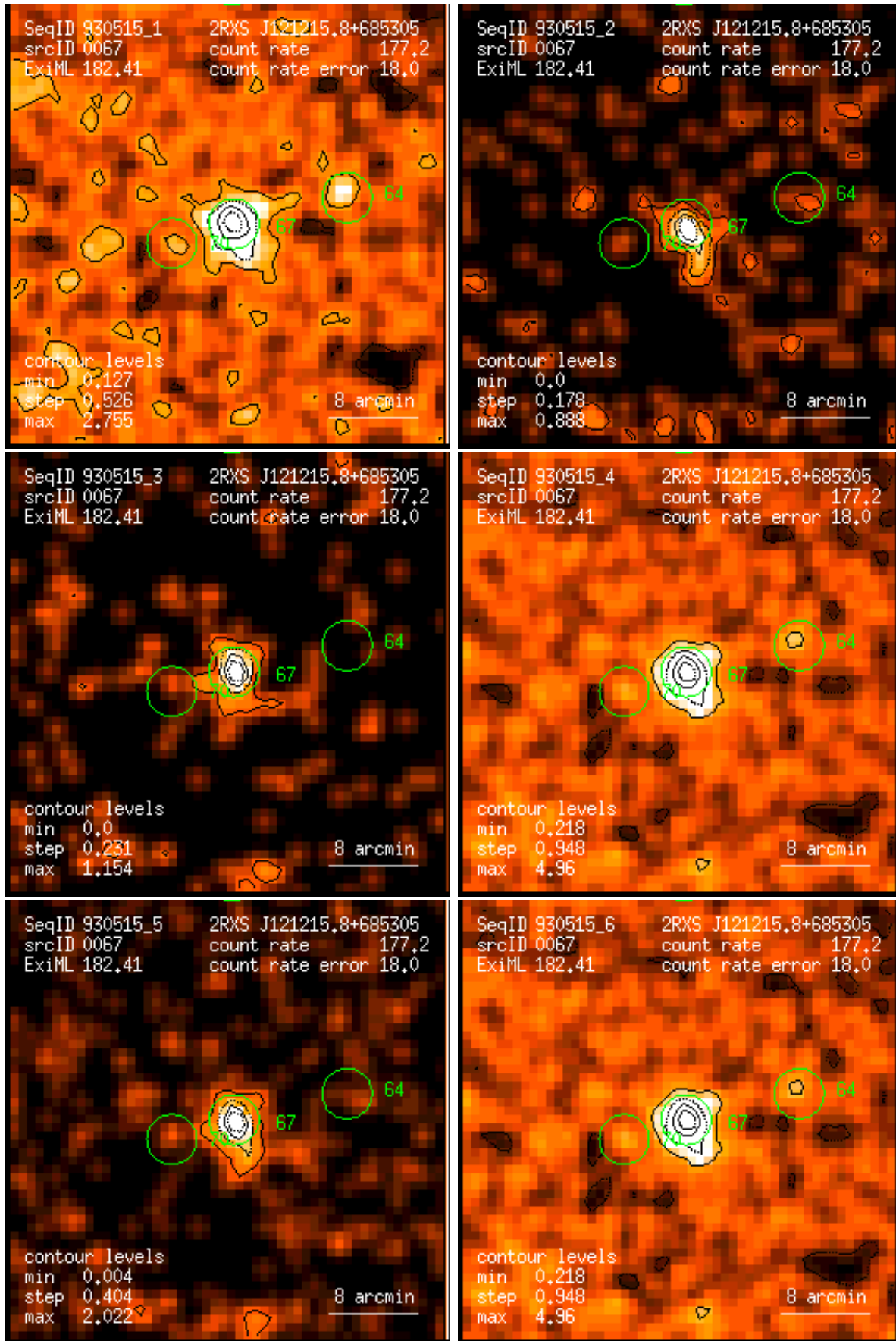
Figure 67: RASS 930515: detection 0067: band rate images, Gaussian filter: (1) PSPC channels 11 – 41, (2) 52 – 90, (3) 91 – 201, (4) 11 – 235, (5) 52 – 201, (6) 11 – 201. Broad band rates in counts/ks. Band rate contour levels in counts/ks/arcmin 2 .
