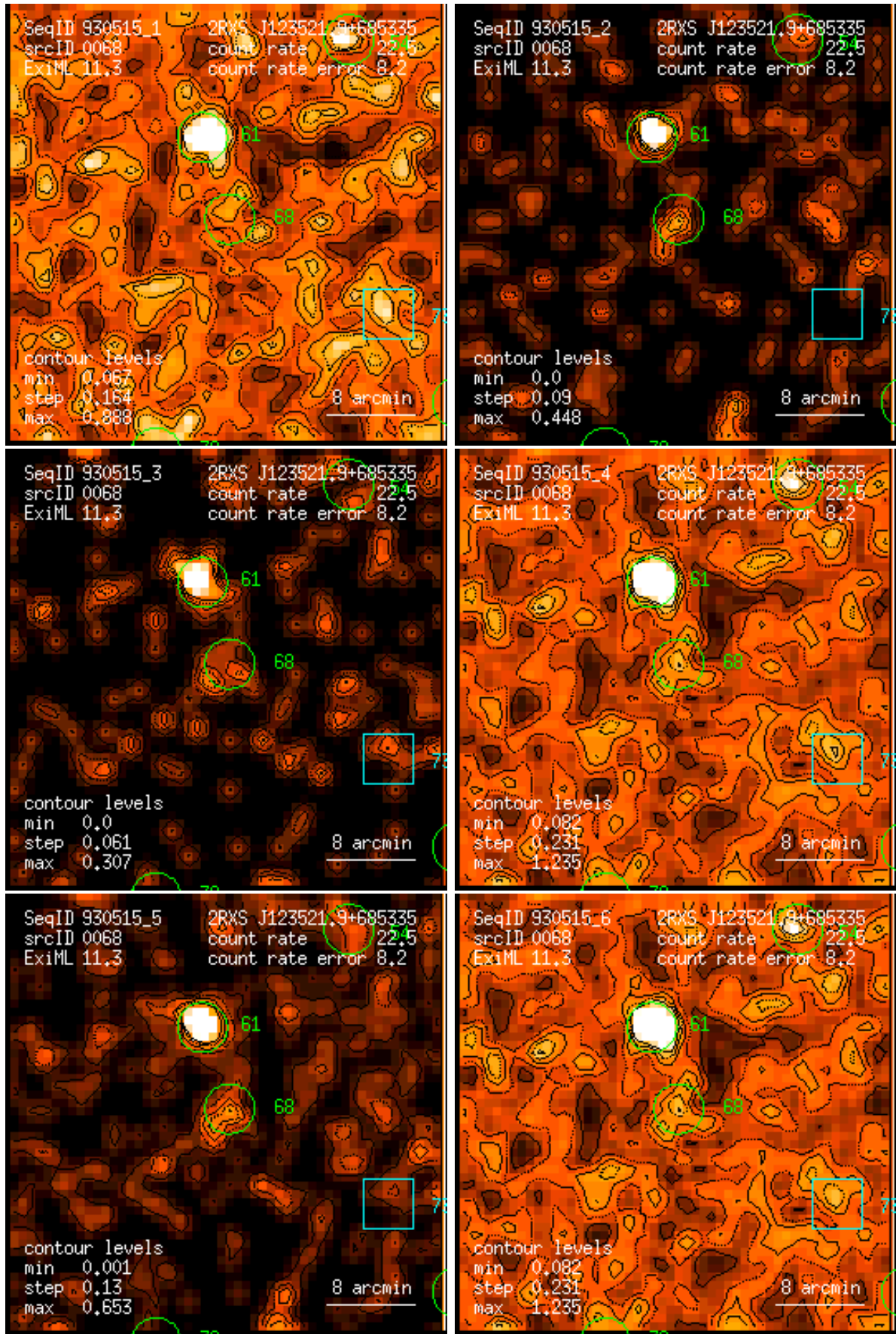
Figure 68: RASS 930515: detection 0068: band rate images, Gaussian filter: (1) PSPC channels 11 – 41, (2) 52 – 90, (3) 91 – 201, (4) 11 – 235, (5) 52 – 201, (6) 11 – 201. Broad band rates in counts/ks. Band rate contour levels in counts/ks/arcmin 2 .
