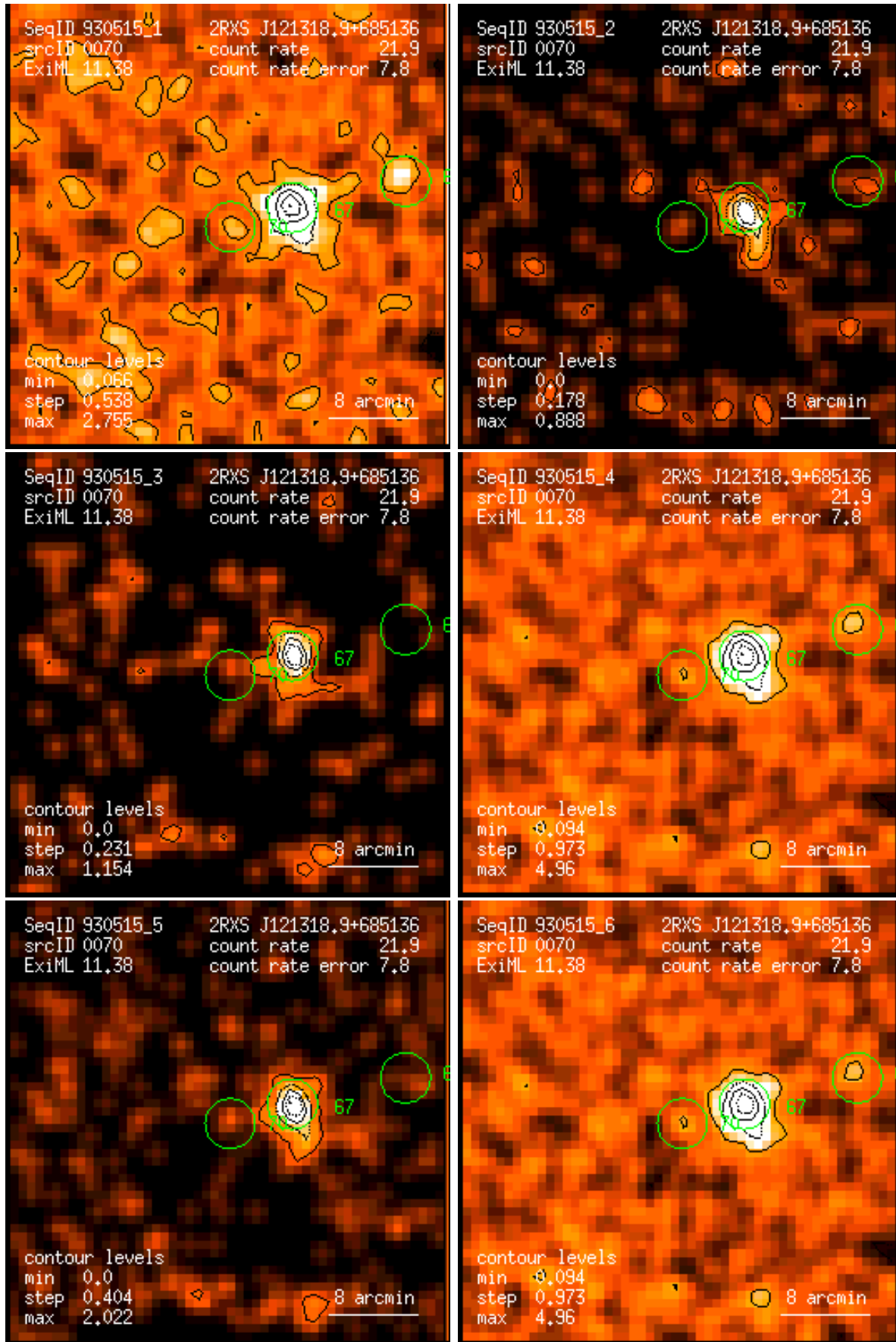
Figure 70: RASS 930515: detection 0070: band rate images, Gaussian filter: (1) PSPC channels 11 – 41, (2) 52 – 90, (3) 91 – 201, (4) 11 – 235, (5) 52 – 201, (6) 11 – 201. Broad band rates in counts/ks. Band rate contour levels in counts/ks/arcmin 2 .
