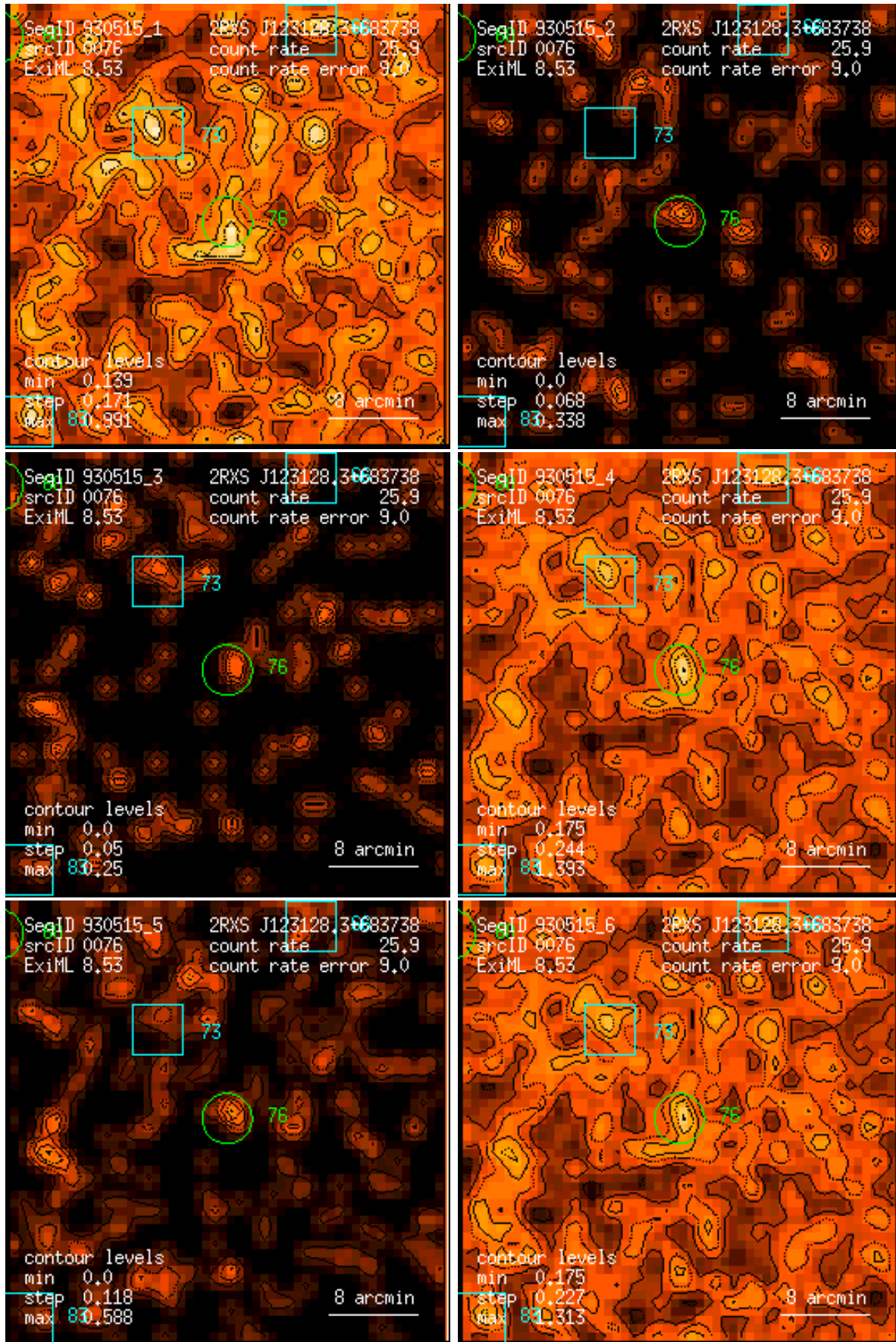
Figure 76: RASS 930515: detection 0076: band rate images, Gaussian filter: (1) PSPC channels 11 – 41, (2) 52 – 90, (3) 91 – 201, (4) 11 – 235, (5) 52 – 201, (6) 11 – 201. Broad band rates in counts/ks. Band rate contour levels in counts/ks/arcmin 2 .
