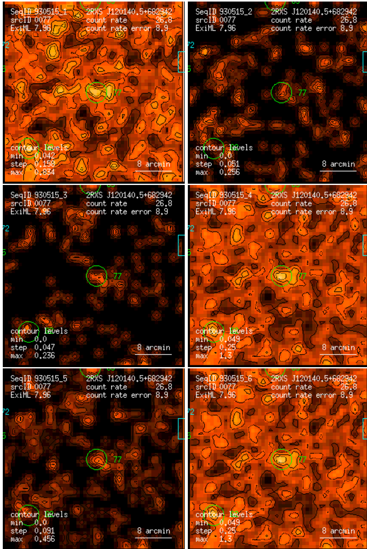
Figure 77: RASS 930515: detection 0077: band rate images, Gaussian filter: (1) PSPC channels 11 – 41, (2) 52 – 90, (3) 91 – 201, (4) 11 – 235, (5) 52 – 201, (6) 11 – 201. Broad band rates in counts/ks. Band rate contour levels in counts/ks/arcmin 2 .
