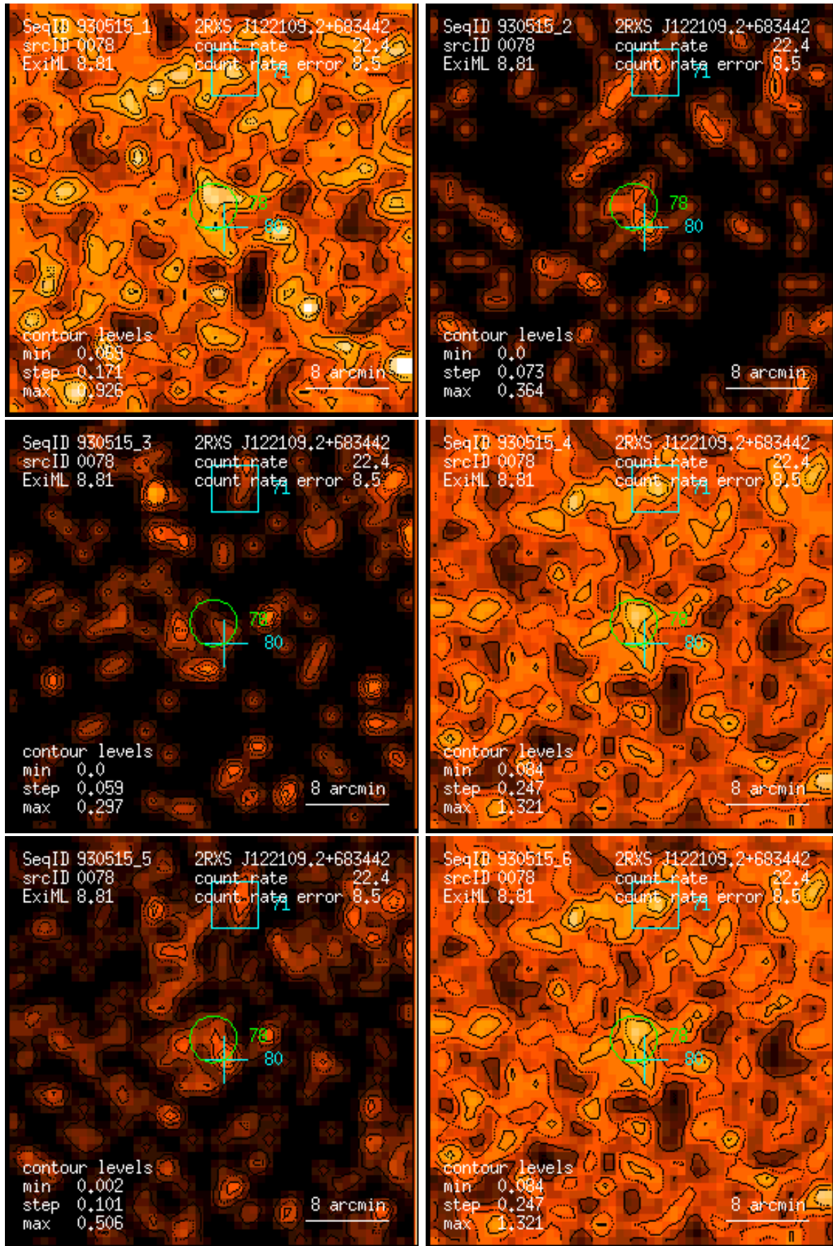
Figure 78: RASS 930515: detection 0078: band rate images, Gaussian filter: (1) PSPC channels 11 – 41, (2) 52 – 90, (3) 91 – 201, (4) 11 – 235, (5) 52 – 201, (6) 11 – 201. Broad band rates in counts/ks. Band rate contour levels in counts/ks/arcmin 2 .
