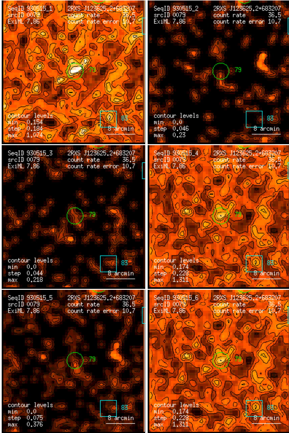
Figure 79: RASS 930515: detection 0079: band rate images, Gaussian filter: (1) PSPC channels 11 – 41, (2) 52 – 90, (3) 91 – 201, (4) 11 – 235, (5) 52 – 201, (6) 11 – 201. Broad band rates in counts/ks. Band rate contour levels in counts/ks/arcmin 2 .
