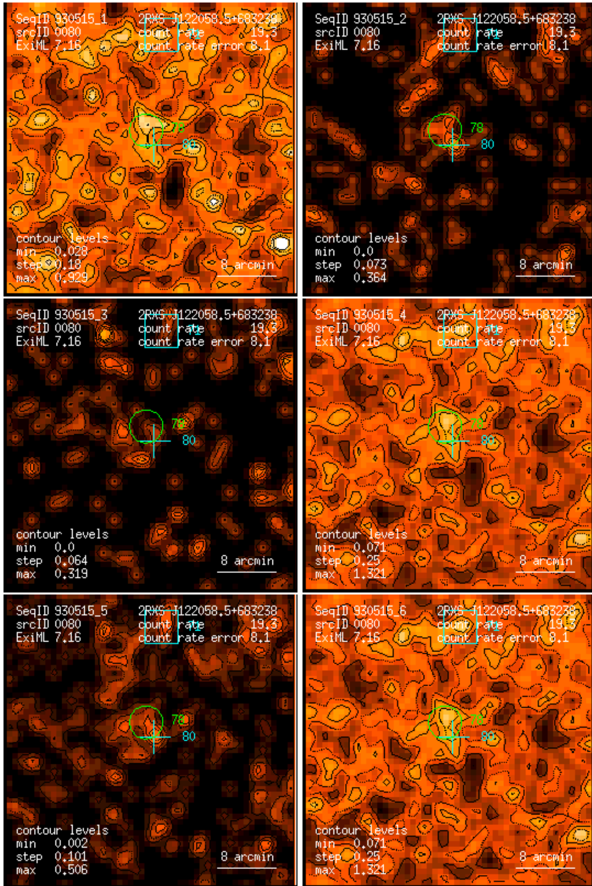
Figure 80: RASS 930515: detection 0080: band rate images, Gaussian filter: (1) PSPC channels 11 – 41, (2) 52 – 90, (3) 91 – 201, (4) 11 – 235, (5) 52 – 201, (6) 11 – 201. Broad band rates in counts/ks. Band rate contour levels in counts/ks/arcmin 2 .
