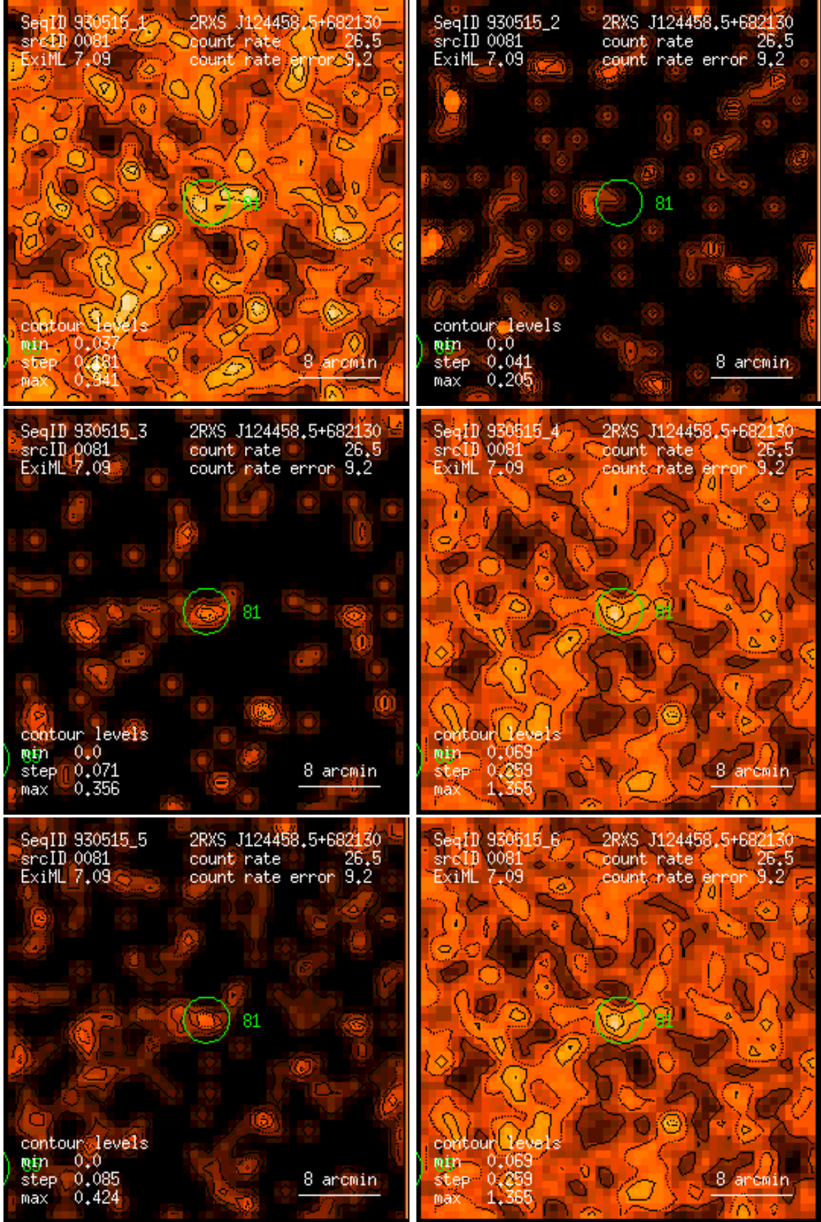
Figure 81: RASS 930515: detection 0081: band rate images, Gaussian filter: (1) PSPC channels 11 – 41, (2) 52 – 90, (3) 91 – 201, (4) 11 – 235, (5) 52 – 201, (6) 11 – 201. Broad band rates in counts/ks. Band rate contour levels in counts/ks/arcmin 2 .
