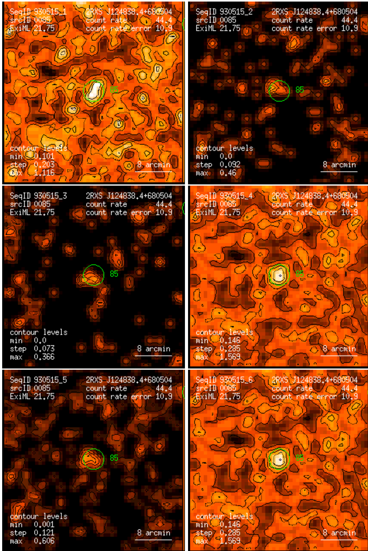
Figure 85: RASS 930515: detection 0085: band rate images, Gaussian filter: (1) PSPC channels 11 – 41, (2) 52 – 90, (3) 91 – 201, (4) 11 – 235, (5) 52 – 201, (6) 11 – 201. Broad band rates in counts/ks. Band rate contour levels in counts/ks/arcmin 2 .
