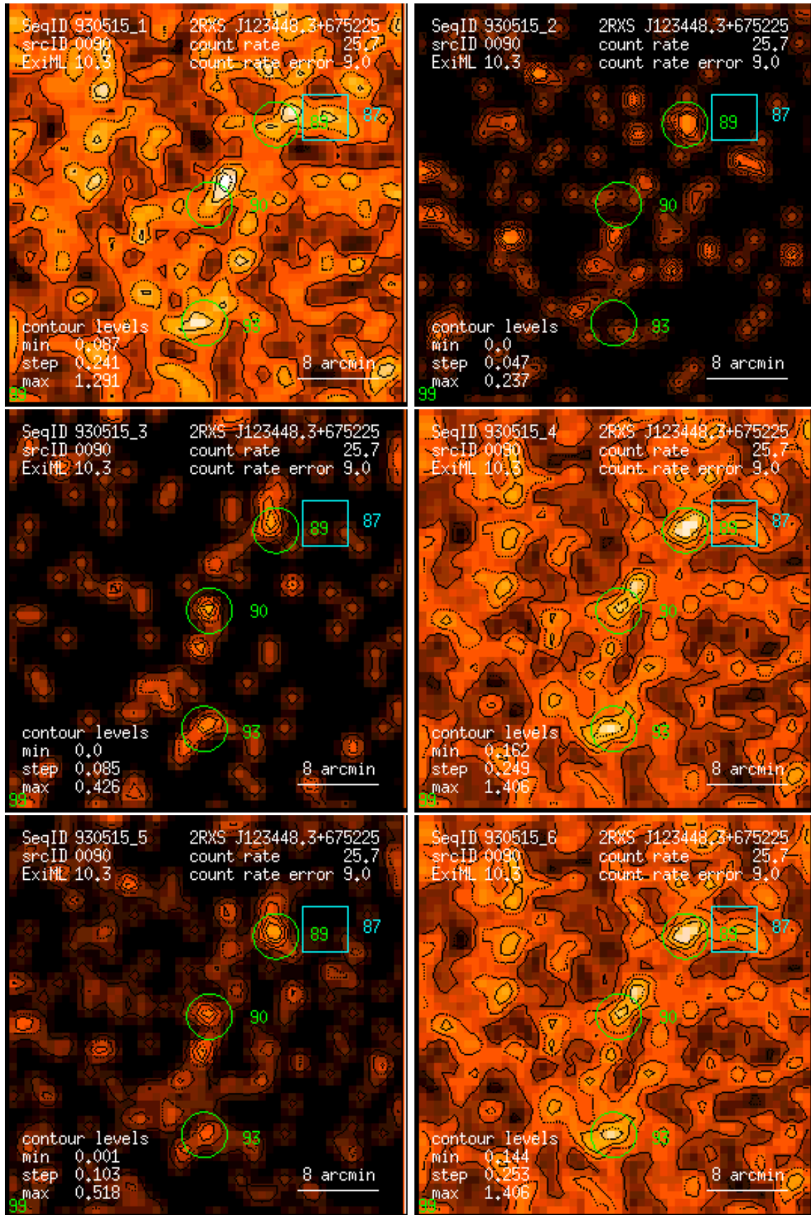
Figure 90: RASS 930515: detection 0090: band rate images, Gaussian filter: (1) PSPC channels 11 – 41, (2) 52 – 90, (3) 91 – 201, (4) 11 – 235, (5) 52 – 201, (6) 11 – 201. Broad band rates in counts/ks. Band rate contour levels in counts/ks/arcmin 2 .
