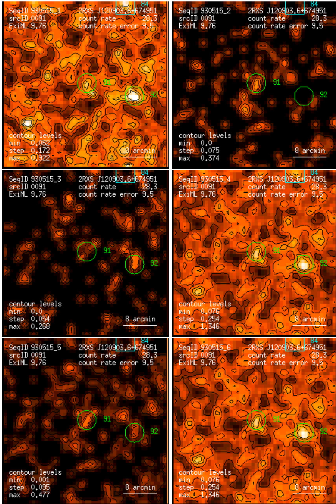
Figure 91: RASS 930515: detection 0091: band rate images, Gaussian filter: (1) PSPC channels 11 – 41, (2) 52 – 90, (3) 91 – 201, (4) 11 – 235, (5) 52 – 201, (6) 11 – 201. Broad band rates in counts/ks. Band rate contour levels in counts/ks/arcmin 2 .
