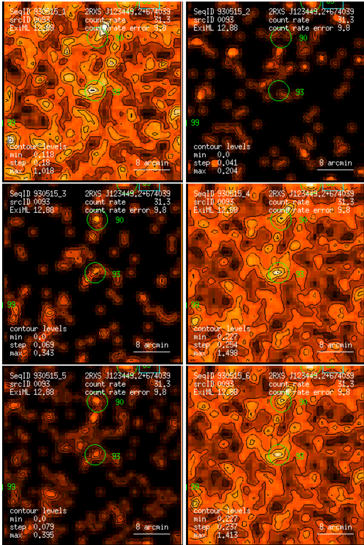
Figure 93: RASS 930515: detection 0093: band rate images, Gaussian filter: (1) PSPC channels 11 – 41, (2) 52 – 90, (3) 91 – 201, (4) 11 – 235, (5) 52 – 201, (6) 11 – 201. Broad band rates in counts/ks. Band rate contour levels in counts/ks/arcmin 2 .
