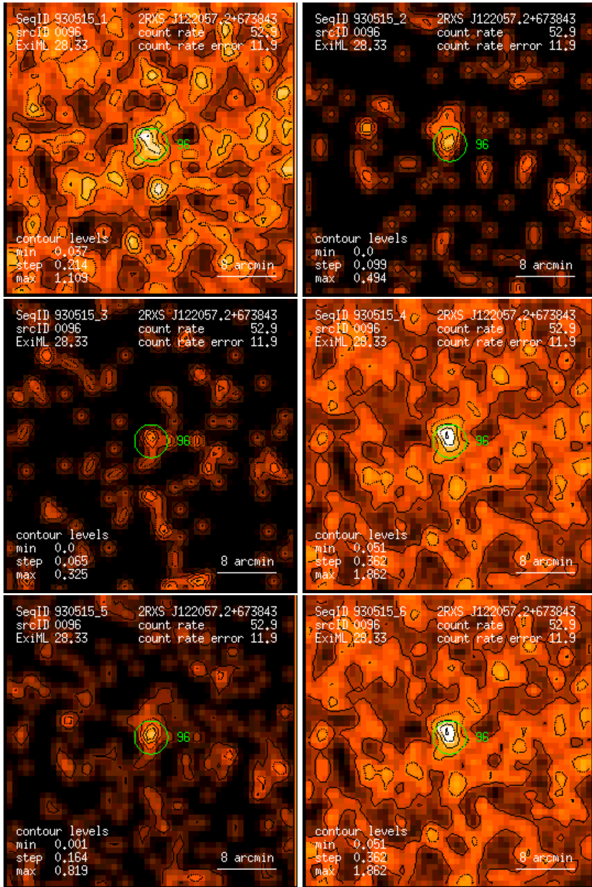
Figure 96: RASS 930515: detection 0096: band rate images, Gaussian filter: (1) PSPC channels 11 – 41, (2) 52 – 90, (3) 91 – 201, (4) 11 – 235, (5) 52 – 201, (6) 11 – 201. Broad band rates in counts/ks. Band rate contour levels in counts/ks/arcmin 2 .
