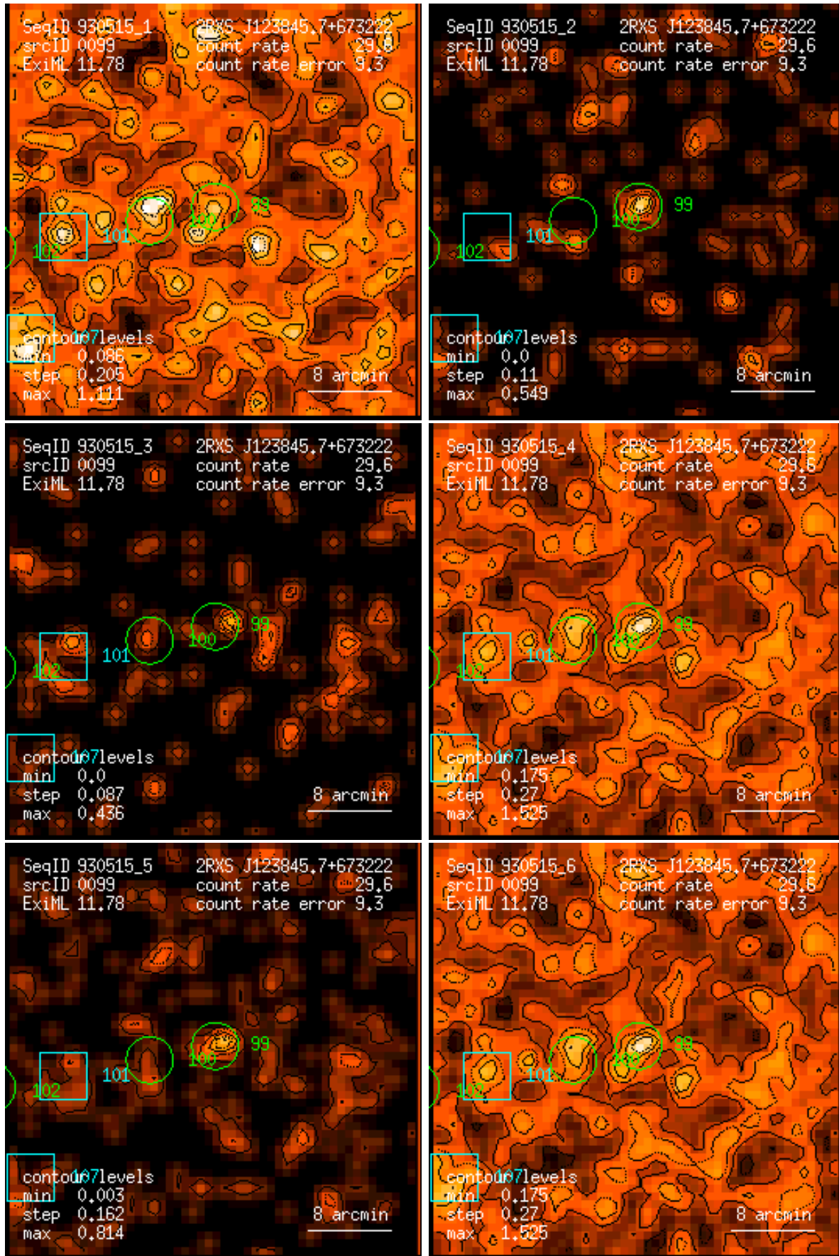
Figure 99: RASS 930515: detection 0099: band rate images, Gaussian filter: (1) PSPC channels 11 – 41, (2) 52 – 90, (3) 91 – 201, (4) 11 – 235, (5) 52 – 201, (6) 11 – 201. Broad band rates in counts/ks. Band rate contour levels in counts/ks/arcmin 2 .
