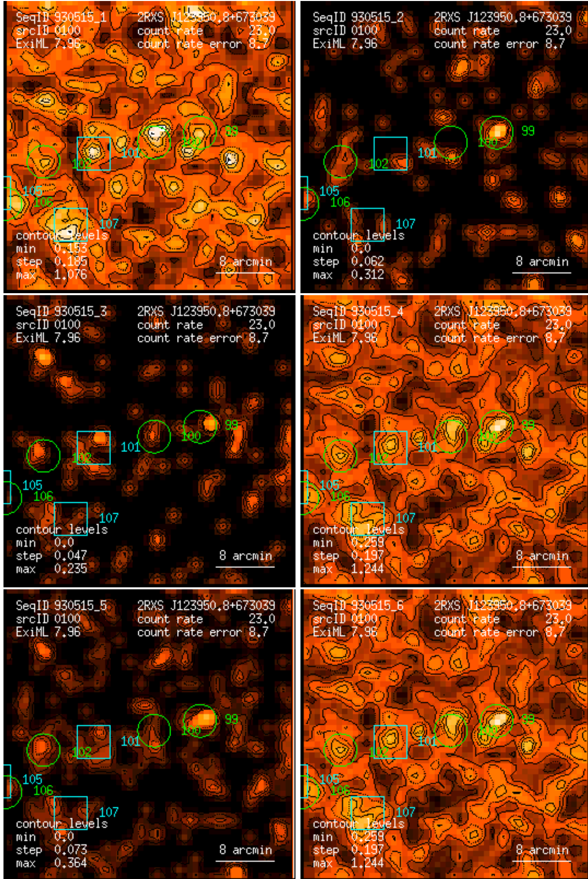
Figure 100: RASS 930515: detection 0100: band rate images, Gaussian filter: (1) PSPC channels 11 – 41, (2) 52 – 90, (3) 91 – 201, (4) 11 – 235, (5) 52 – 201, (6) 11 – 201. Broad band rates in counts/ks. Band rate contour levels in counts/ks/arcmin 2 .
