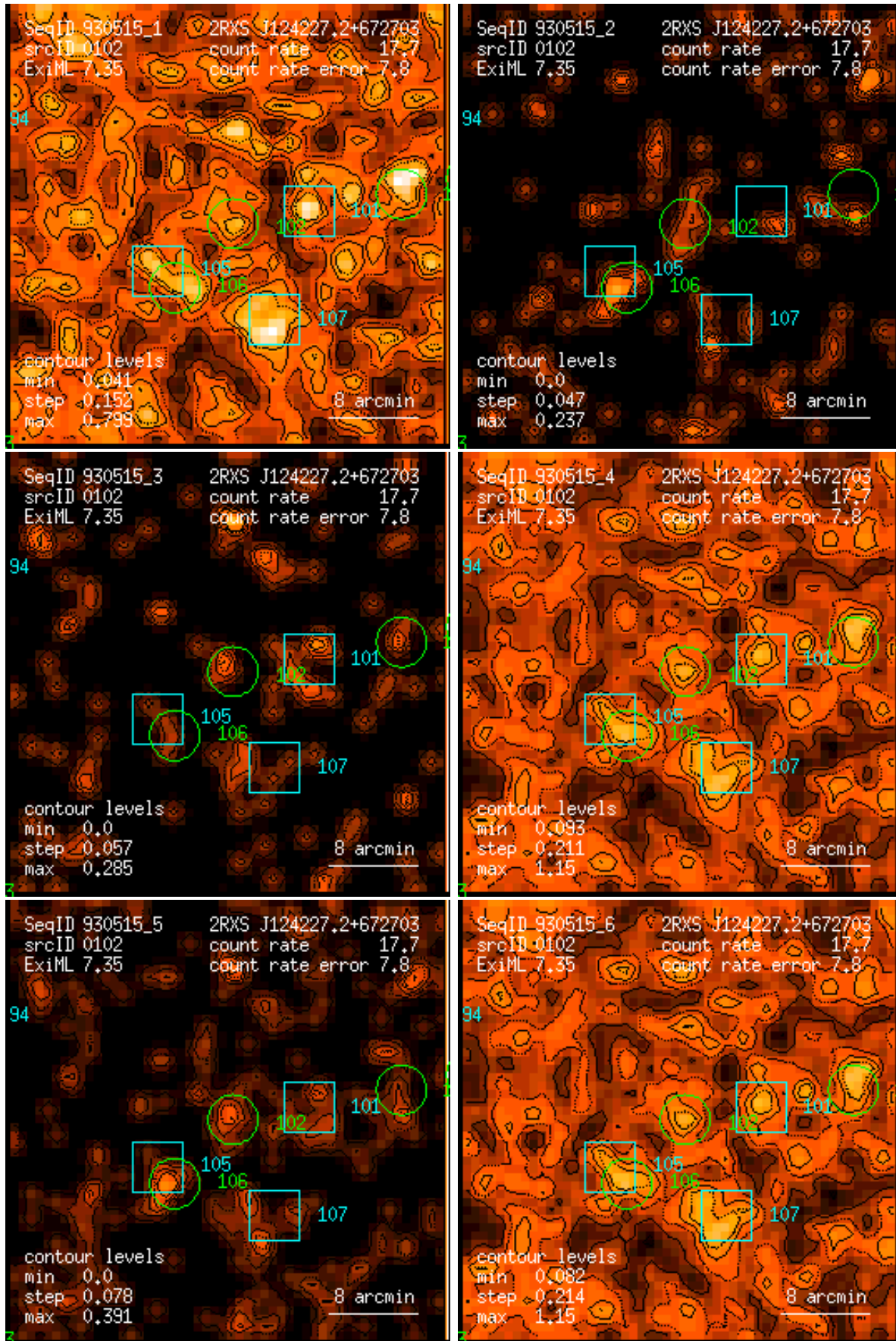
Figure 102: RASS 930515: detection 0102: band rate images, Gaussian filter: (1) PSPC channels 11 – 41, (2) 52 – 90, (3) 91 – 201, (4) 11 – 235, (5) 52 – 201, (6) 11 – 201. Broad band rates in counts/ks. Band rate contour levels in counts/ks/arcmin 2 .
