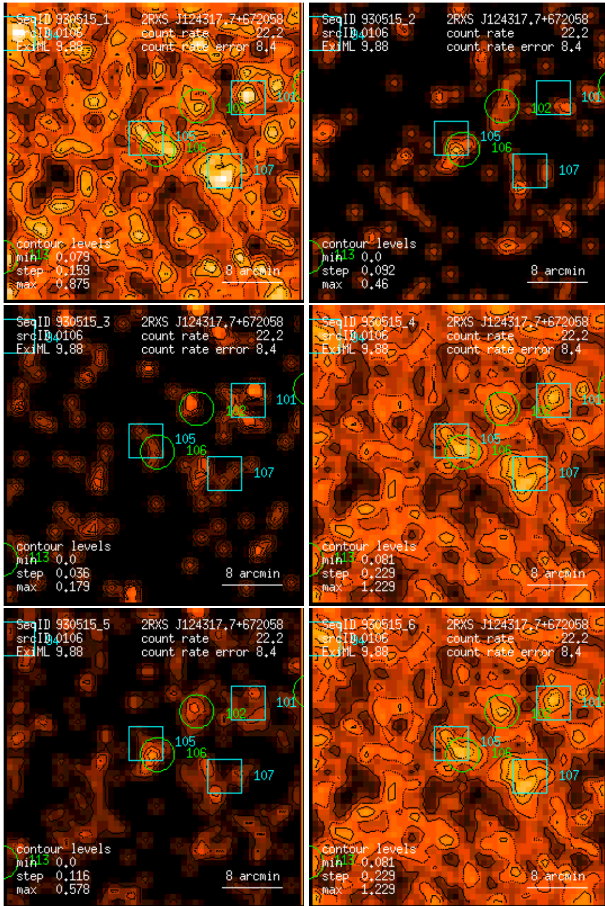
Figure 106: RASS 930515: detection 0106: band rate images, Gaussian filter: (1) PSPC channels 11 – 41, (2) 52 – 90, (3) 91 – 201, (4) 11 – 235, (5) 52 – 201, (6) 11 – 201. Broad band rates in counts/ks. Band rate contour levels in counts/ks/arcmin 2 .
