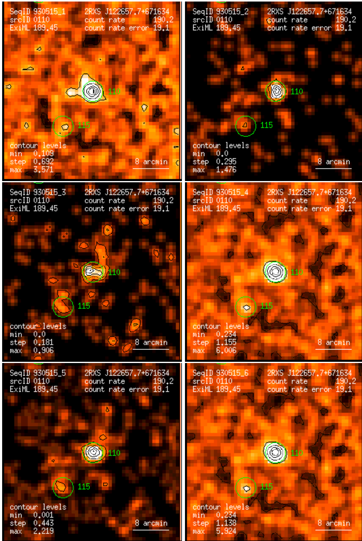
Figure 110: RASS 930515: detection 0110: band rate images, Gaussian filter: (1) PSPC channels 11 – 41, (2) 52 – 90, (3) 91 – 201, (4) 11 – 235, (5) 52 – 201, (6) 11 – 201. Broad band rates in counts/ks. Band rate contour levels in counts/ks/arcmin 2 .
