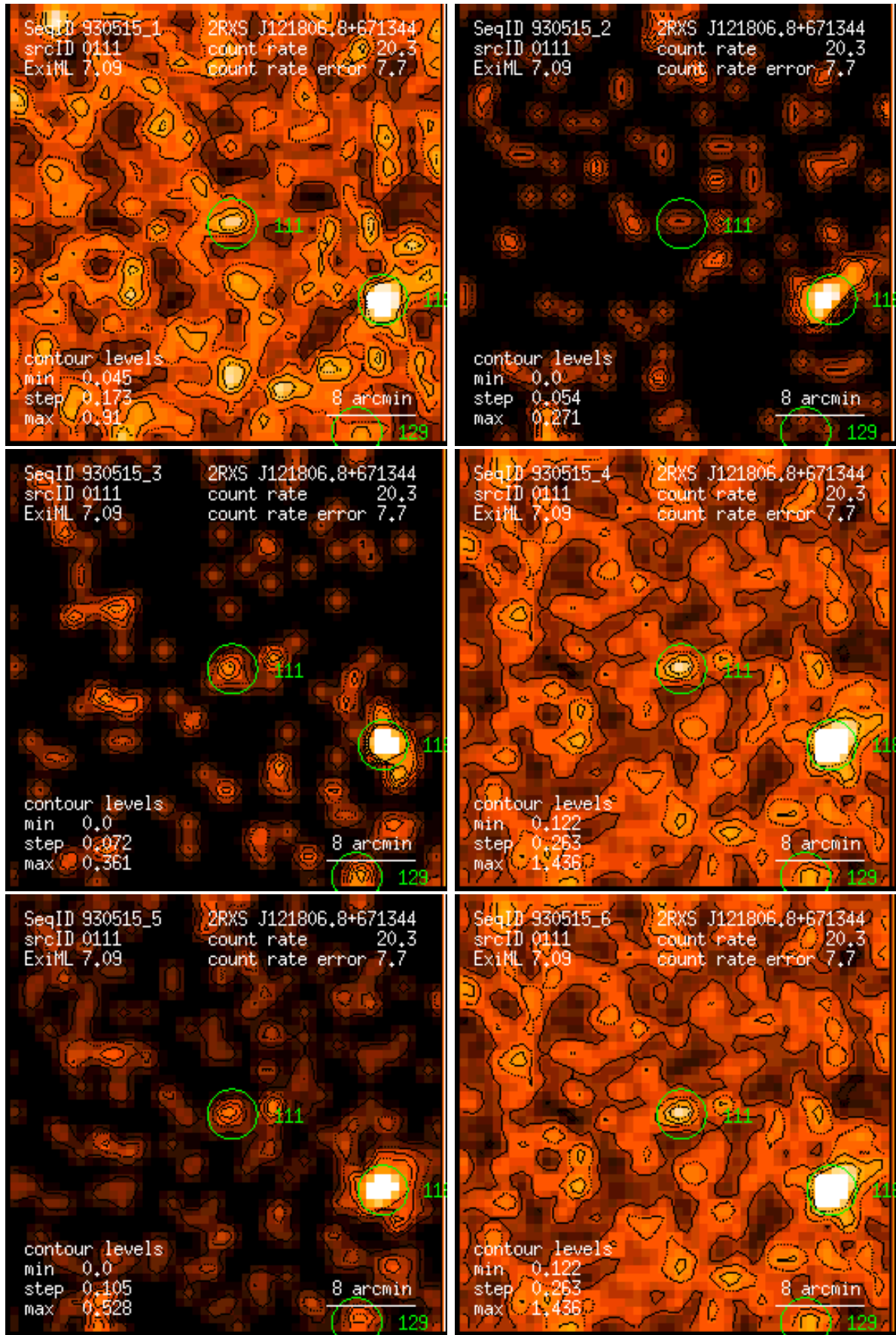
Figure 111: RASS 930515: detection 0111: band rate images, Gaussian filter: (1) PSPC channels 11 – 41, (2) 52 – 90, (3) 91 – 201, (4) 11 – 235, (5) 52 – 201, (6) 11 – 201. Broad band rates in counts/ks. Band rate contour levels in counts/ks/arcmin 2 .
