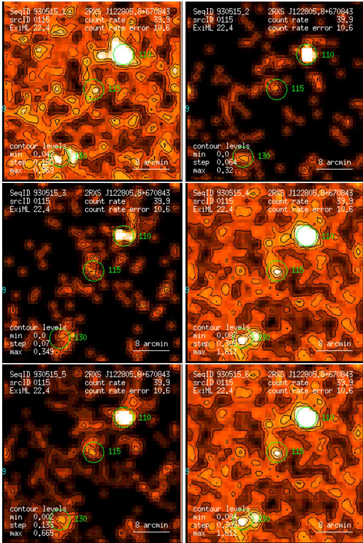
Figure 115: RASS 930515: detection 0115: band rate images, Gaussian filter: (1) PSPC channels 11 – 41, (2) 52 – 90, (3) 91 – 201, (4) 11 – 235, (5) 52 – 201, (6) 11 – 201. Broad band rates in counts/ks. Band rate contour levels in counts/ks/arcmin 2 .
