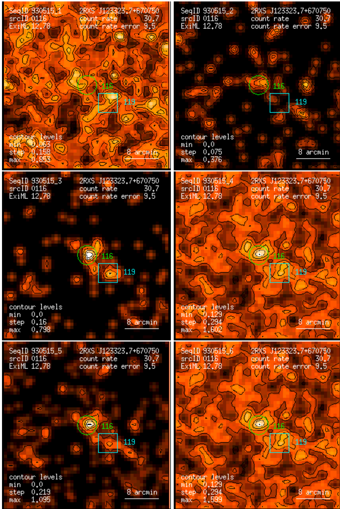
Figure 116: RASS 930515: detection 0116: band rate images, Gaussian filter: (1) PSPC channels 11 – 41, (2) 52 – 90, (3) 91 – 201, (4) 11 – 235, (5) 52 – 201, (6) 11 – 201. Broad band rates in counts/ks. Band rate contour levels in counts/ks/arcmin 2 .
