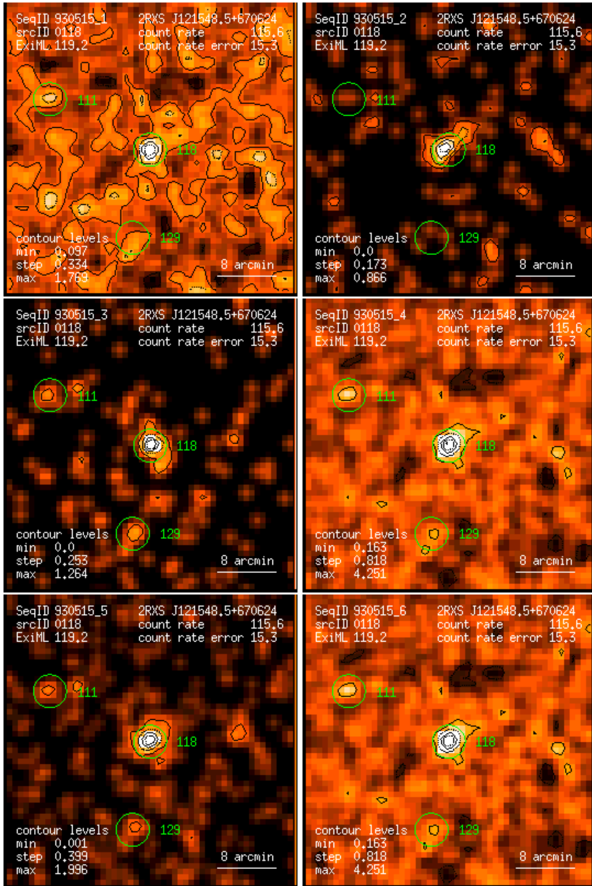
Figure 118: RASS 930515: detection 0118: band rate images, Gaussian filter: (1) PSPC channels 11 – 41, (2) 52 – 90, (3) 91 – 201, (4) 11 – 235, (5) 52 – 201, (6) 11 – 201. Broad band rates in counts/ks. Band rate contour levels in counts/ks/arcmin 2 .
